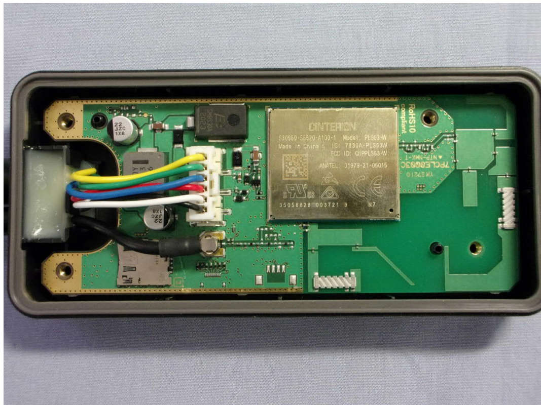
Rear open 2
