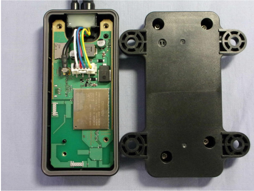
Rear open 2
