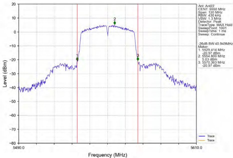
802.11n(HT40)_MCH_5550MHz_Ant22_NTNV
