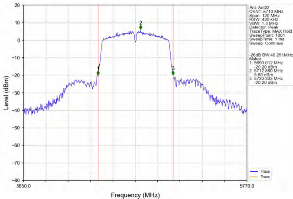
802.11n(HT40)_HCH_5710MHz_Ant22_NTNV
