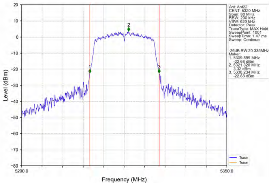
802.11ac(VHT20)_HCH_5320MHz_Ant22_NTNV
