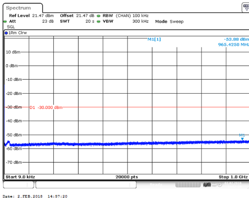
Figure 219 Spurious Emissions (9 kHz – 1 GHz) – 256QAM (5765.0/ 5785.0/ 5805.0 MHz) (3 X 20MHz Channel BW)
