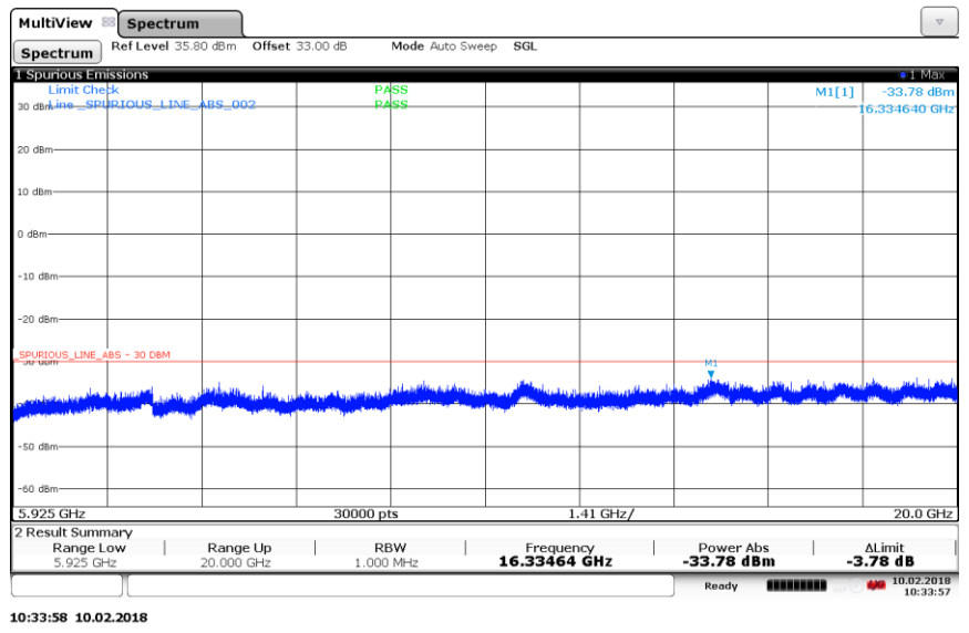
Figure 201 Spurious Emissions (5.925 GHz – 20 GHz) – 64QAM (5765.0/ 5805.0 MHz) (2 X 20MHz Channel BW)
