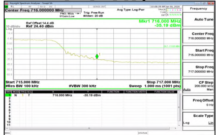
LTE\Band17_10MHz_QPSK_50_0_HighCH23800-711
