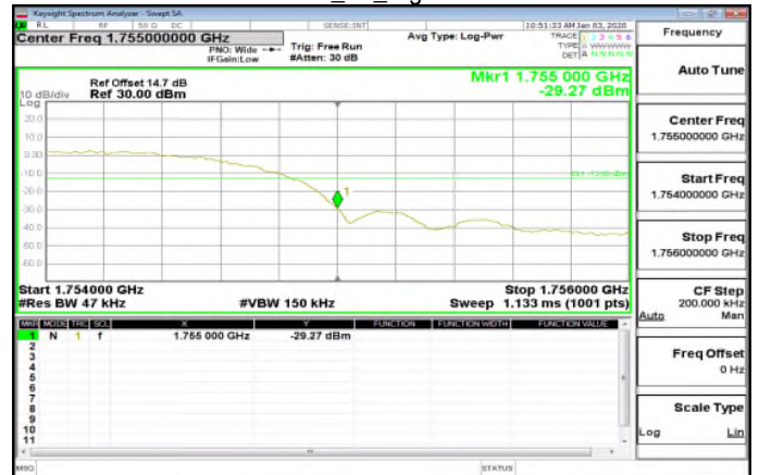
HSDPA\HSDPA_B4_HighCH1513-1752.6
