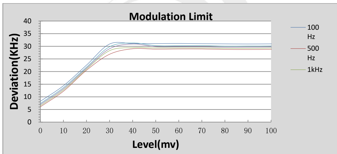
Modulation Deviation of Mid Channel
