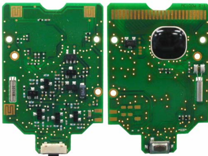
Main unit
