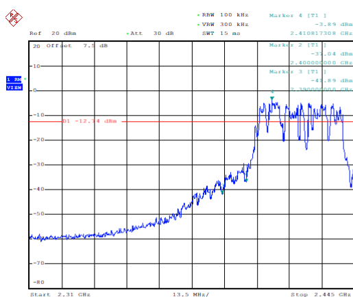
Band Edges (802.11n-40MHz, Ch3)
