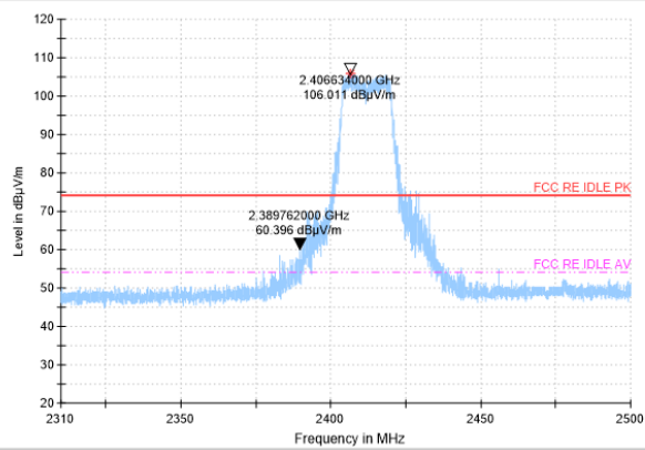
Peak detector
