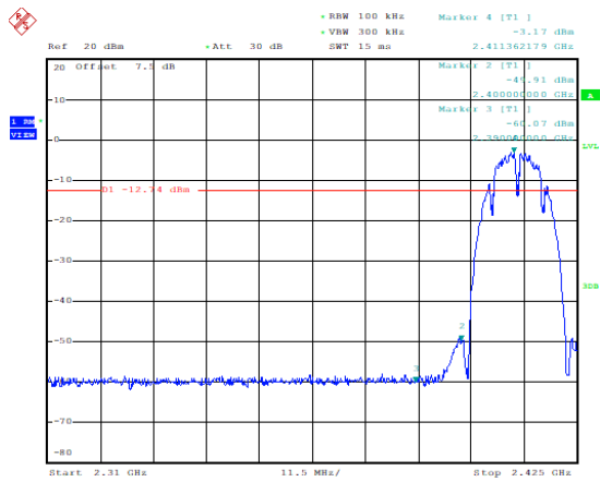
Band Edges (802.11b, Ch1)
