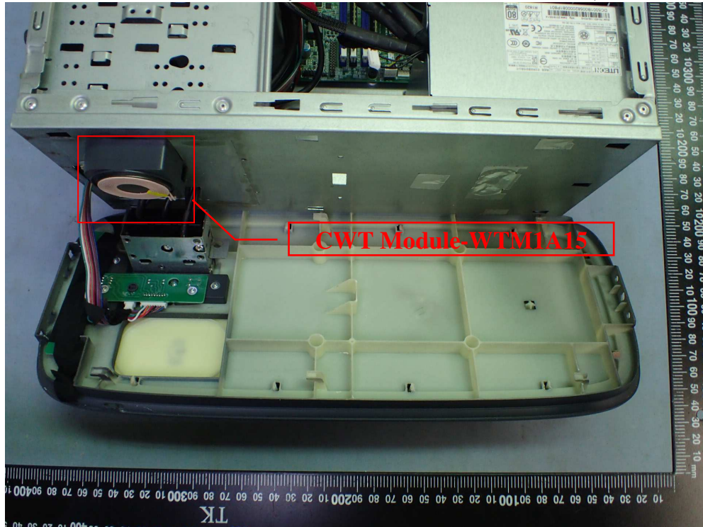
Figure 11 Personal Computer D19E4, Internal View (Removed Cover)
