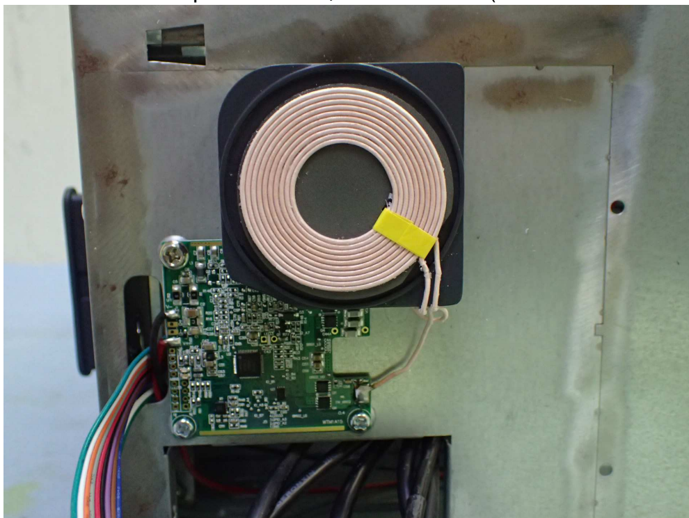
Figure 12 Personal Computer D19E4, Internal View (CWT Module-WTM1A15)
