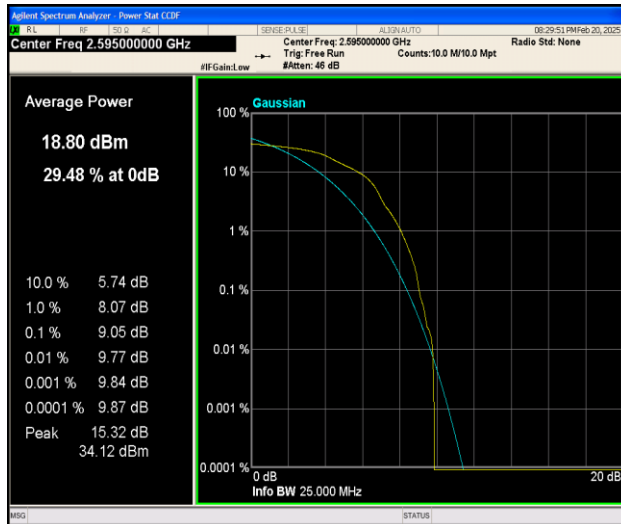
Band38-10MHz-16QAM-38000-1RB#0-PASS
