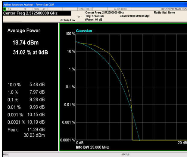
Band38-5MHz-16QAM-37775-25RB#0-PASS
