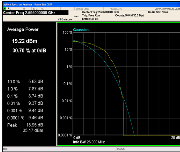
Band38-15MHz-16QAM-38000-1RB#0-PASS
