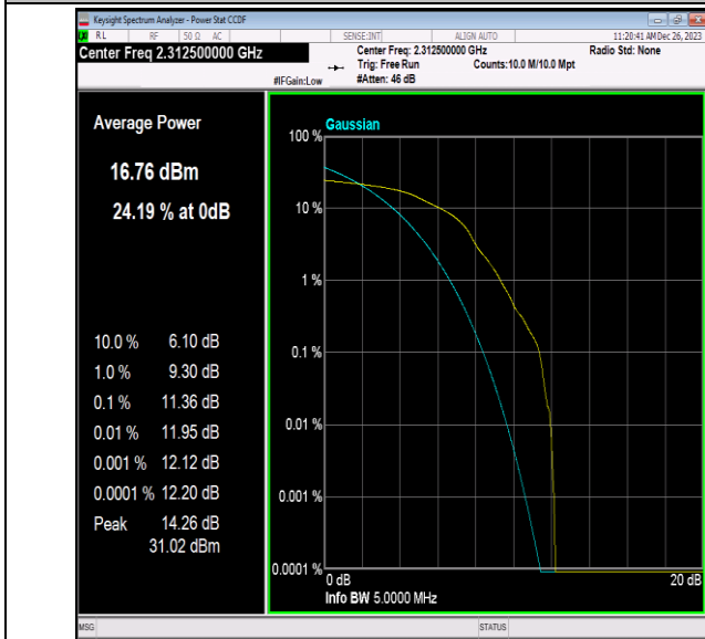
40(2305-2315)-5MHz-16QAM-38775-1RB#0-PASS
