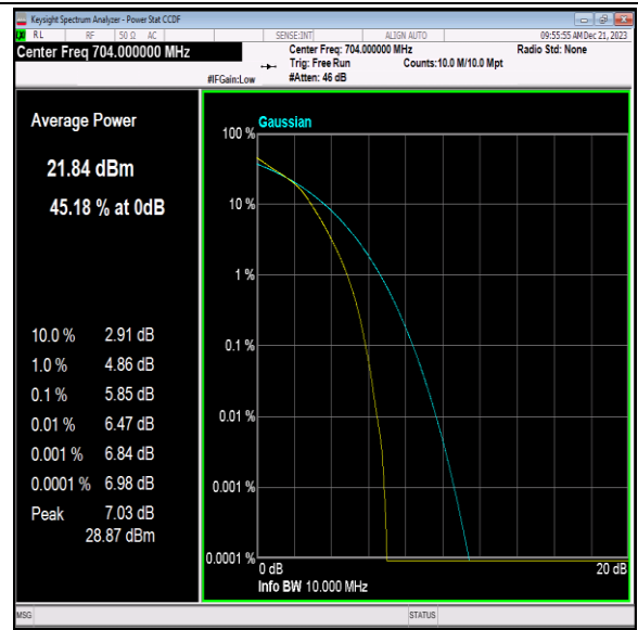
Band12-10MHz-16QAM-23060-50RB#0-PASS
