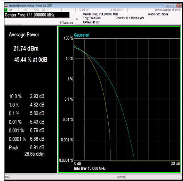
Band12-10MHz-16QAM-23130-50RB#0-PASS
