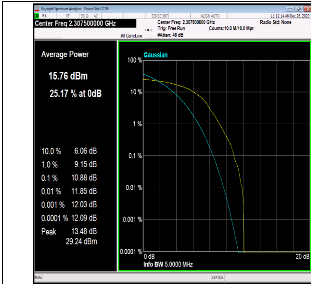
40(2305-2315)-5MHz-64QAM-38725-1RB#0-PASS
