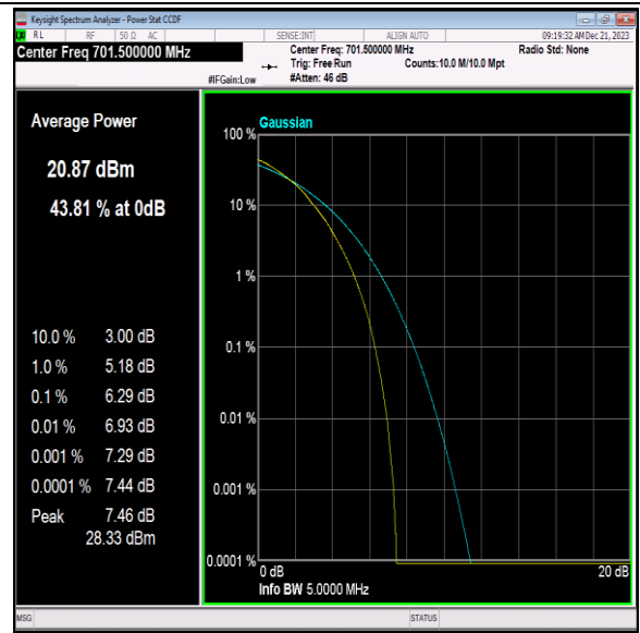
Band12-5MHz-64QAM-23035-25RB#0-PASS
