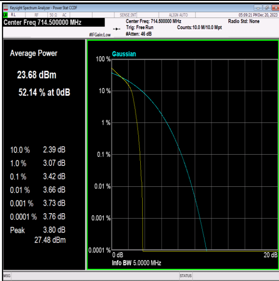
Band12-3MHz-QPSK-23165-1RB#0-PASS
