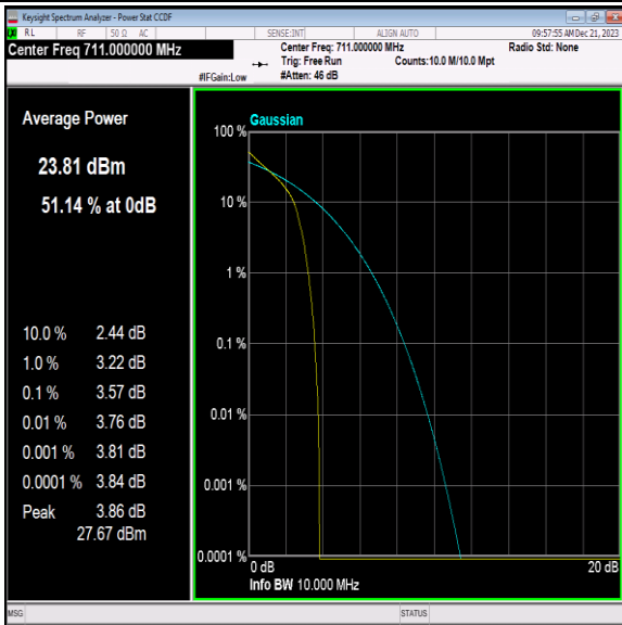
Band12-10MHz-QPSK-23130-1RB#0-PASS
