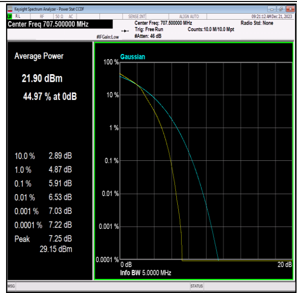
Band12-5MHz-16QAM-23095-25RB#0-PASS
