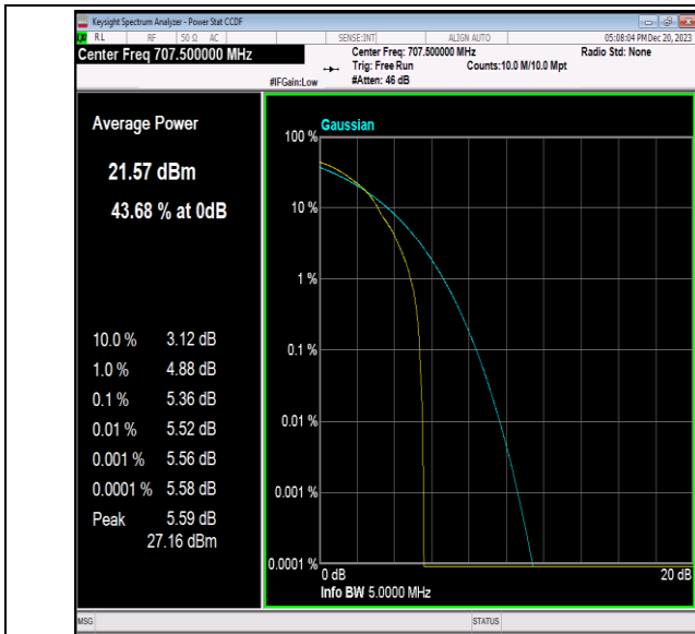
Band12-3MHz-64QAM-23095-1RB#0-PASS
