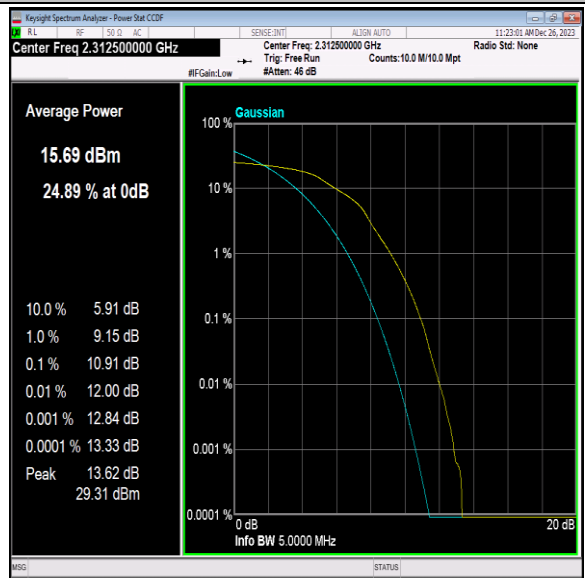
40(2305-2315)-5MHz-16QAM-38775-25RB#0-PASS
