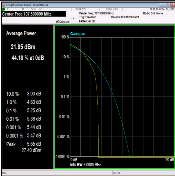
Band12-5MHz-64QAM-23095-1RB#0-PASS
