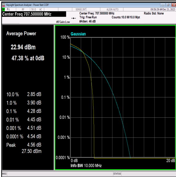
Band12-10MHz-16QAM-23095-1RB#0-PASS
