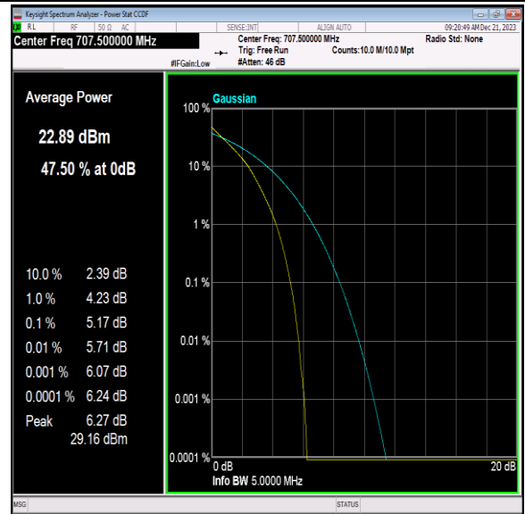
Band12-5MHz-QPSK-23095-25RB#0-PASS
