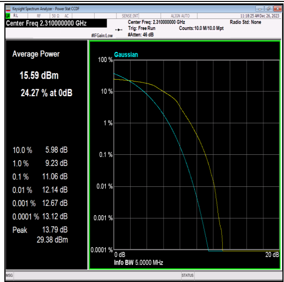
40(2305-2315)-5MHz-16QAM-38750-25RB#0-PASS
