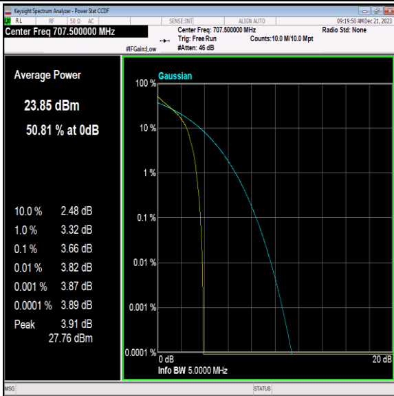
Band12-5MHz-QPSK-23095-1RB#0-PASS
