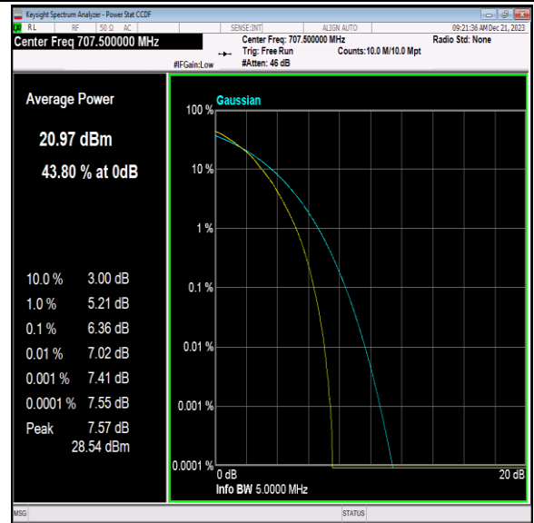
Band12-5MHz-64QAM-23095-25RB#0-PASS
