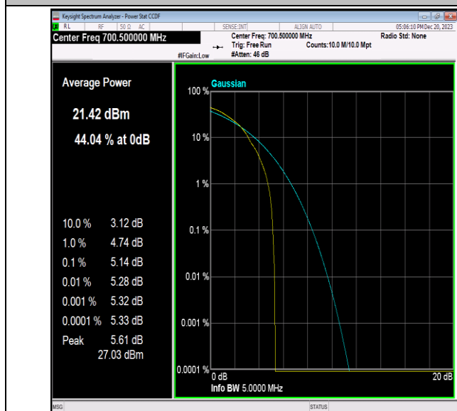
Band12-3MHz-64QAM-23025-1RB#0-PASS
