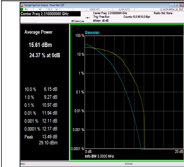
40(2305-2315)-5MHz-64QAM-38750-1RB#0-PASS
