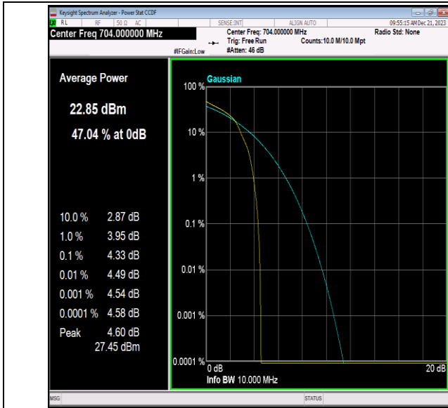
Band12-10MHz-16QAM-23060-1RB#0-PASS
