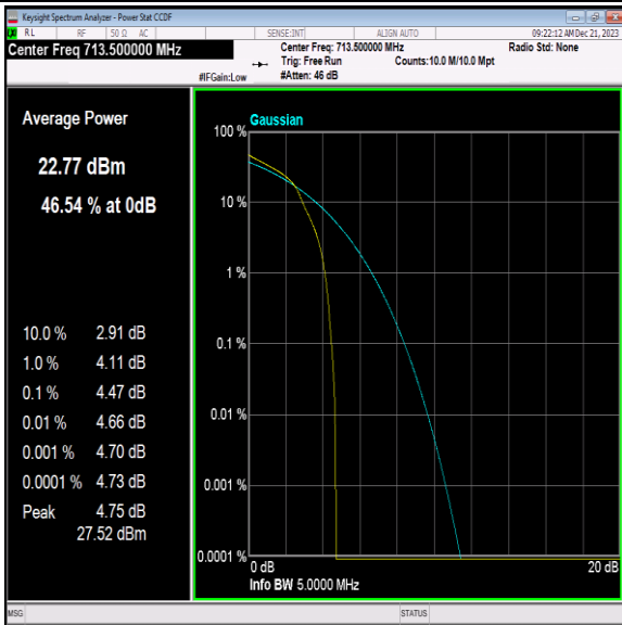
Band12-5MHz-16QAM-23155-1RB#0-PASS
