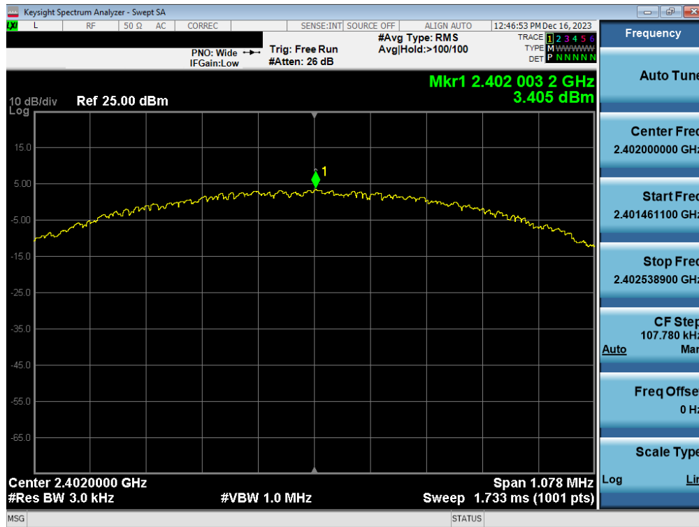
Plot 7-37. Power Spectral Density Plot Antenna WF7b (Bluetooth (LE), 1Mbps, ePA – Ch. 0)
