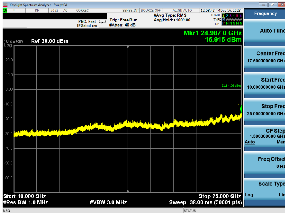
Plot 7-72. Conducted Spurious Plot Antenna WF7b (Bluetooth (LE), 1Mbps, ePA – Ch. 19)
