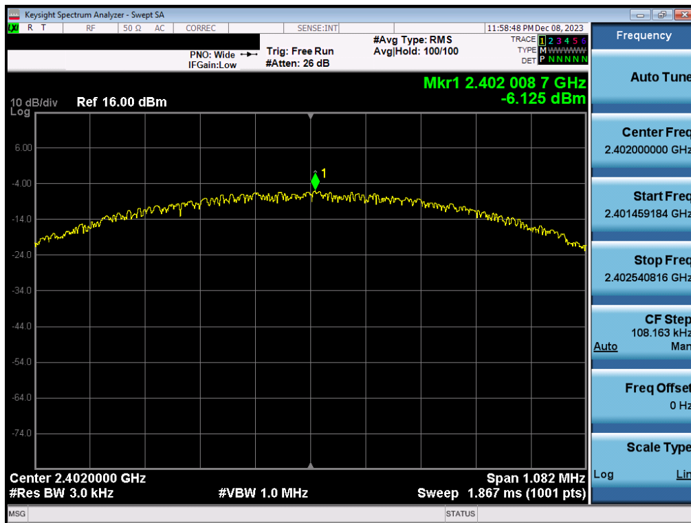
Plot 7-28. Power Spectral Density Plot Antenna WF2b (Bluetooth (LE), 1Mbps, iPA – Ch. 0)
