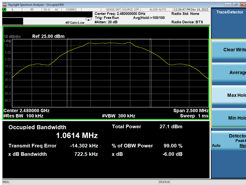
Plot 7-3. 6dB BW & 99% OBW Plot Antenna WF7b (Bluetooth (LE), 1Mbps, ePA – Ch. 39)
