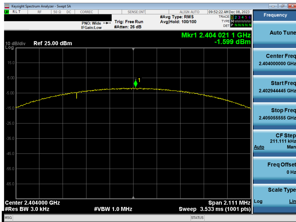
Plot 7-50. Power Spectral Density Plot Antenna WF2b (Bluetooth (LE), 2Mbps, ePA – Ch. 1)
