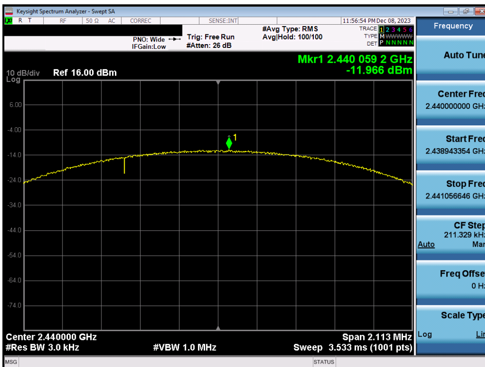
Plot 7-58. Power Spectral Density Plot Antenna WF2b (Bluetooth (LE), 2Mbps, iPA – Ch. 19)
