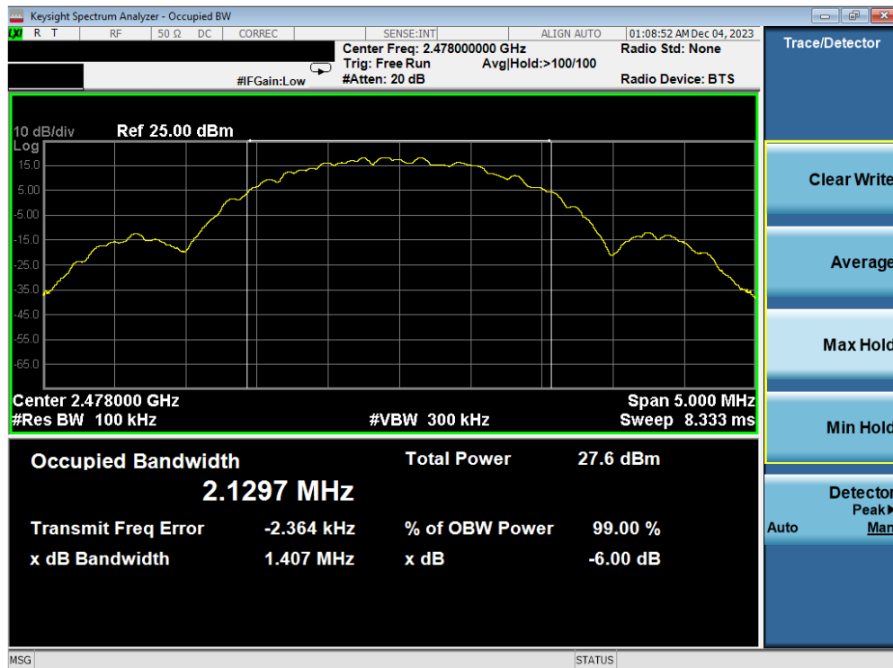
Plot 7-12. 6dB BW & 99% OBW Plot Antenna WF2b (Bluetooth (LE), 2Mbps, ePA – Ch. 38)
