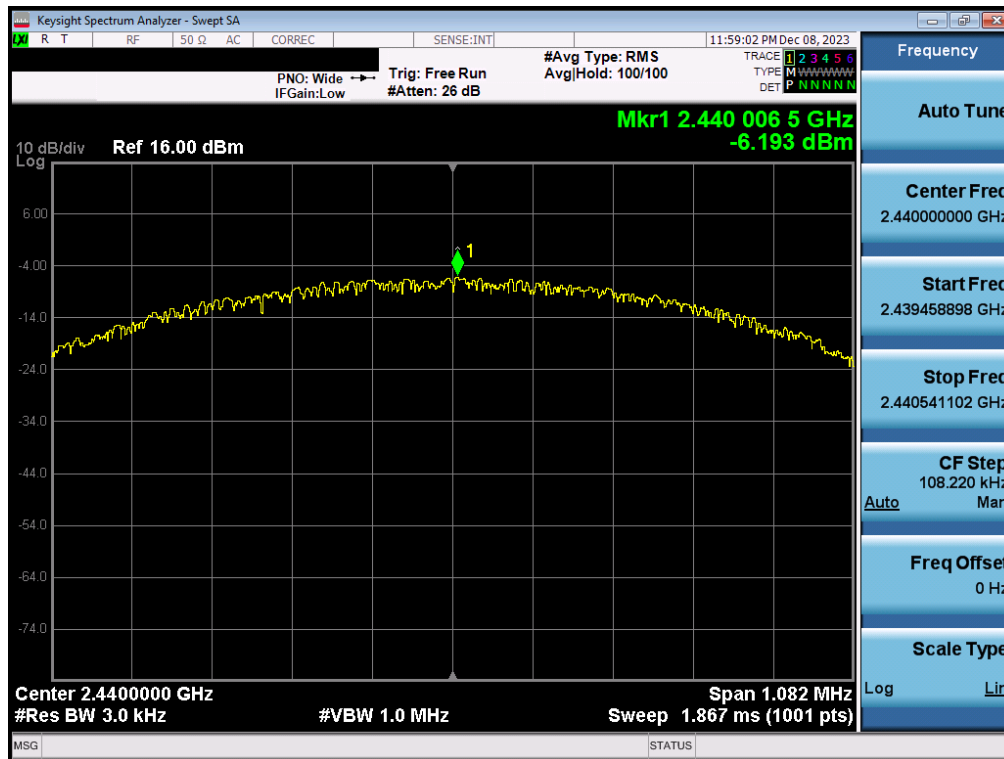
Plot 7-29. Power Spectral Density Plot Antenna WF2b (Bluetooth (LE), 1Mbps, iPA – Ch. 19)
