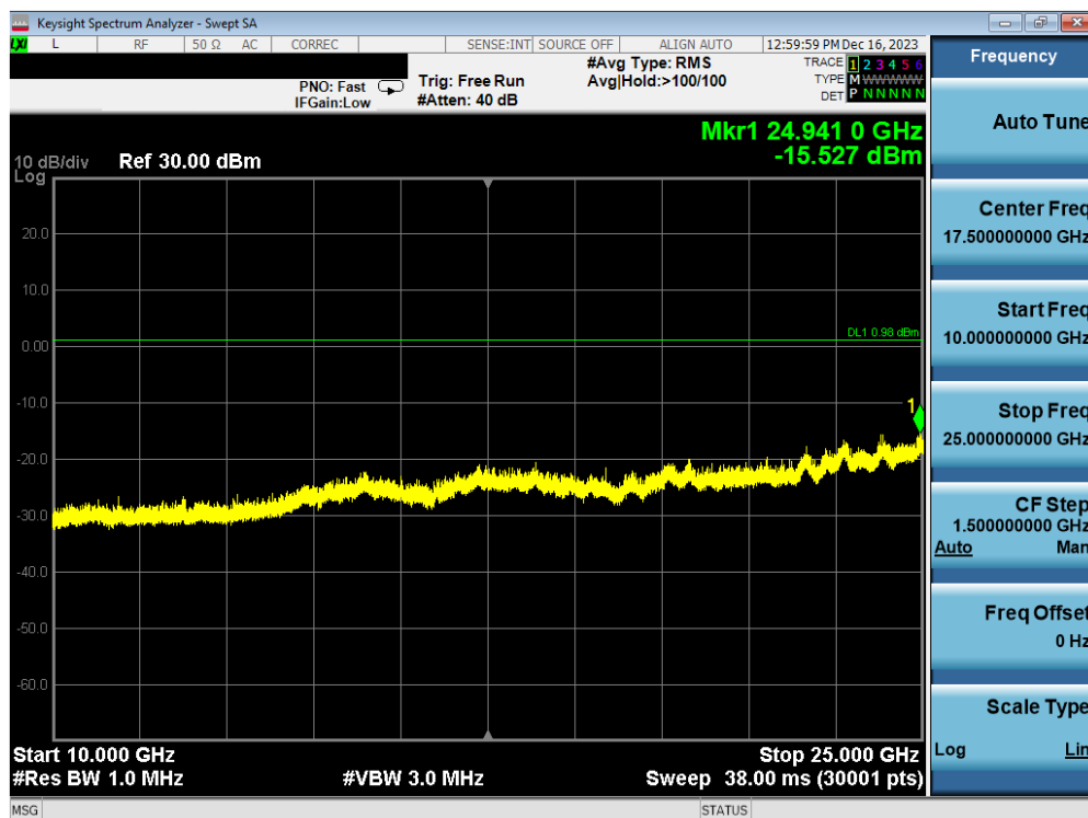
Plot 7-74. Conducted Spurious Plot Antenna WF7b (Bluetooth (LE), 1Mbps, ePA – Ch. 39)
