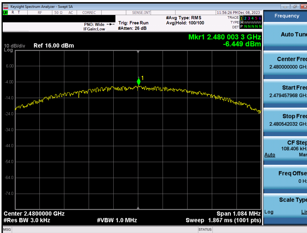
Plot 7-48. Power Spectral Density Plot Antenna WF2b (Bluetooth (LE), 1Mbps, iPA – Ch. 39)
