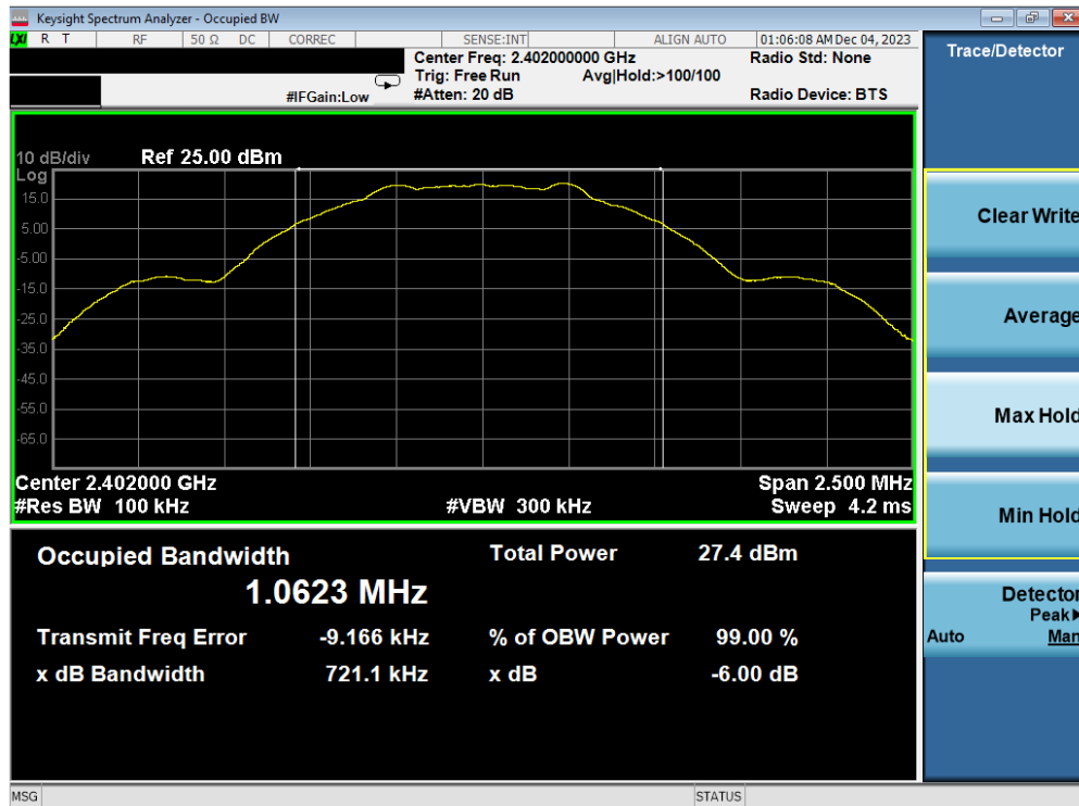
Plot 7-7. 6dB BW & 99% OBW Plot Antenna WF2b (Bluetooth (LE), 1Mbps, ePA – Ch. 0)
