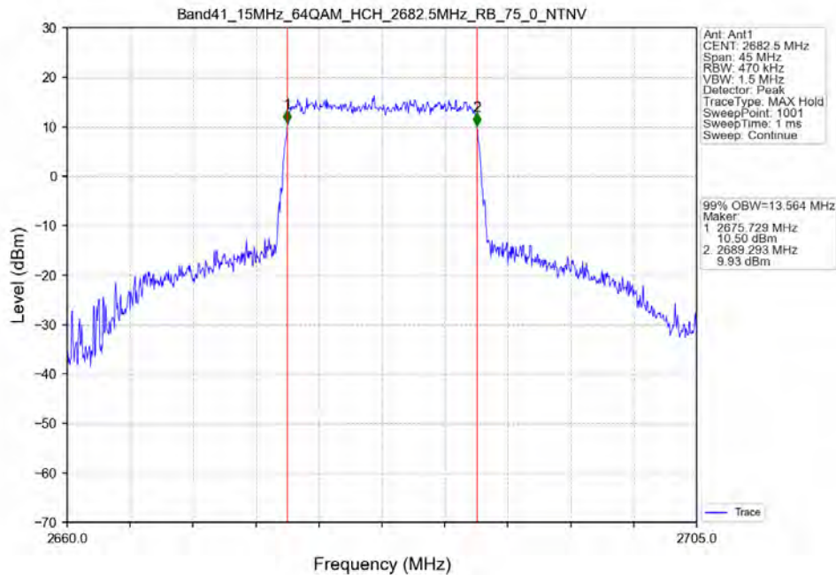
Band41_15MHz_64QAM_HCH_2682.5MHz_RB_75_0_NTNV
