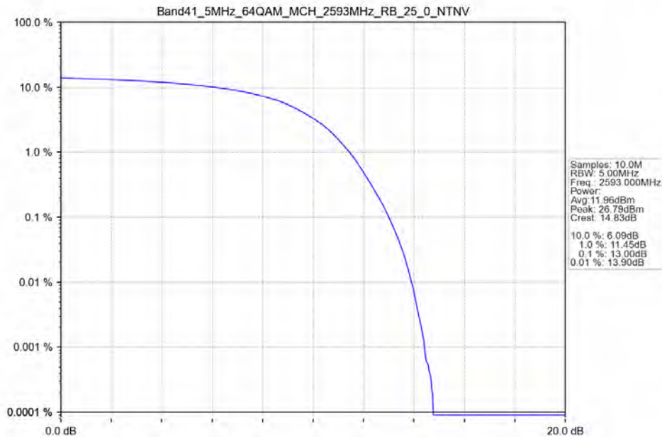
Band41_5MHz_64QAM_MCH_2593MHz_RB_25_0_NTNV
