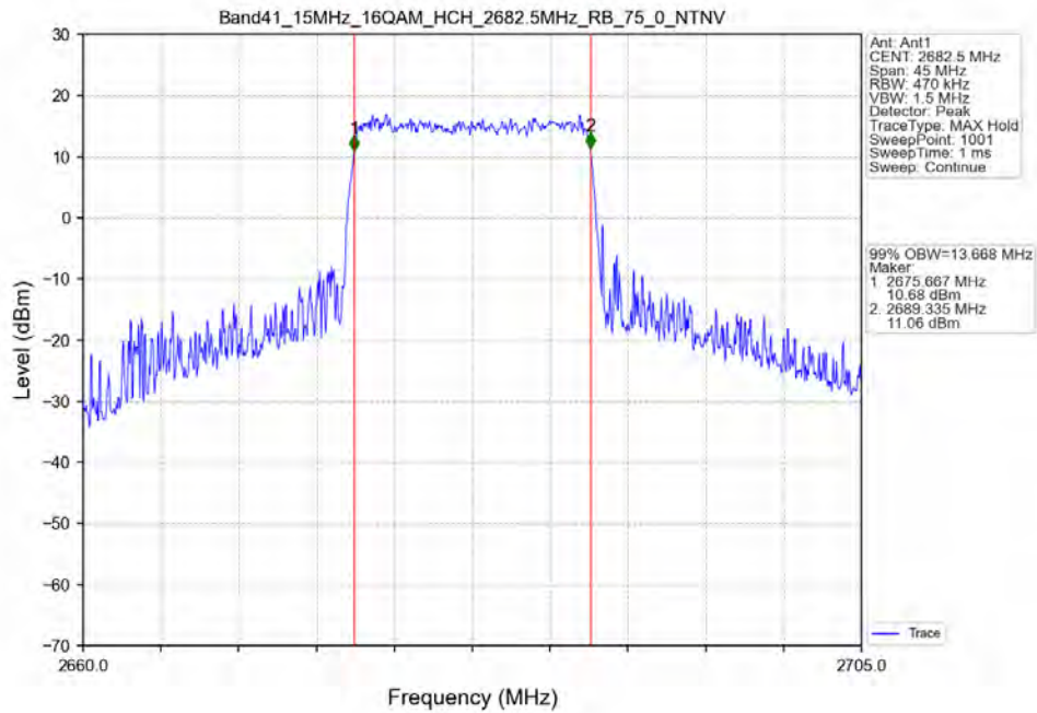
Band41_15MHz_16QAM_HCH_2682.5MHz_RB_75_0_NTNV
