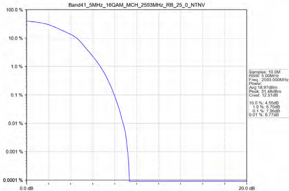
Band41_5MHz_16QAM_MCH_2593MHz_RB_25_0_NTNV
