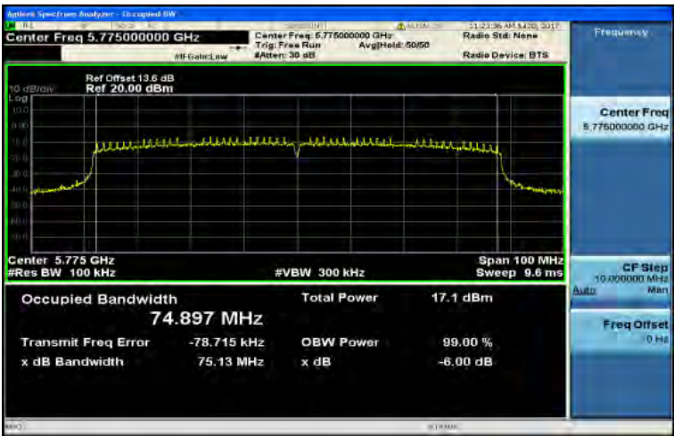
802.11ac_VHT80, 5725~5850 MHz 6dB Band Width Test Data CH-Low (5775 MHz)
