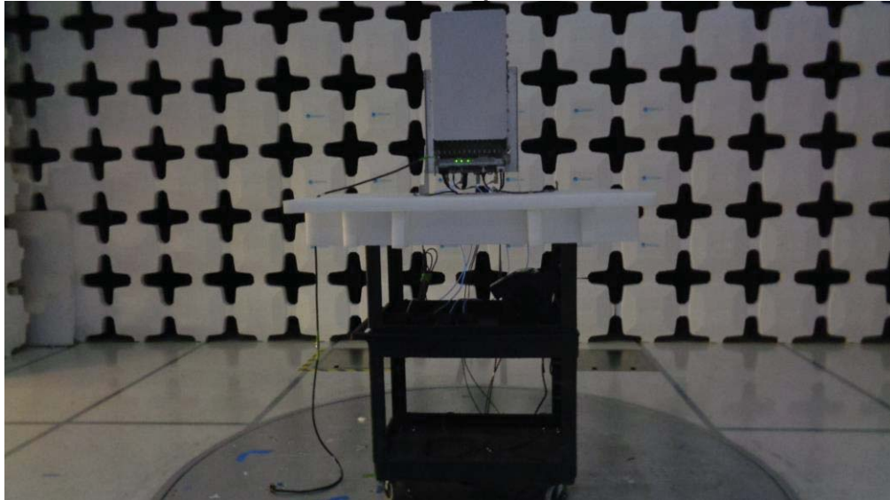
Radiated Spurious
