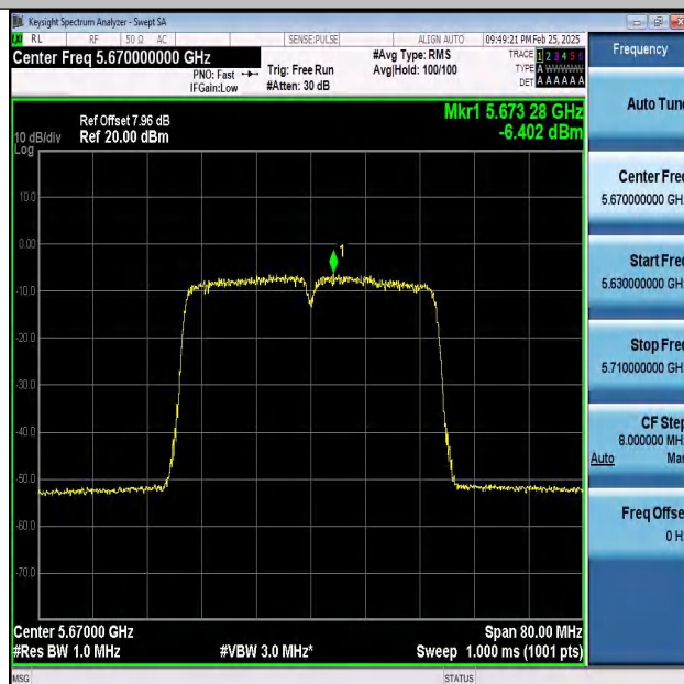
11N40MIMO-Ant2-5670-PASS
