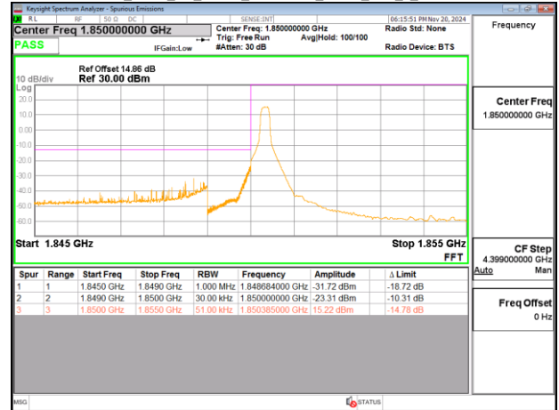
Band2_5MHz_CP_OFDM_SCS15kHz_QPSK_RB25_0_CH370500
