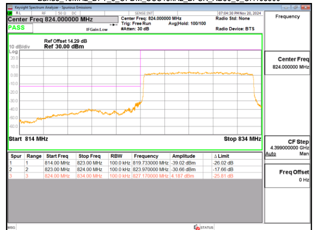
Band5_10MHz_DFT_s_OFDM_SCS15kHz_BPSK_RB50_0_CH165800
