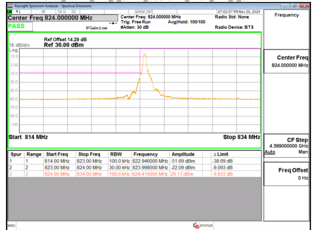
Band5_10MHz_DFT_s_OFDM_SCS15kHz_BPSK_RB50_0_CH165800
