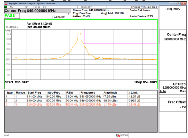
Band5_5MHz_DFT_s_OFDM_SCS15kHz_BPSK_RB25_0_CH169300
