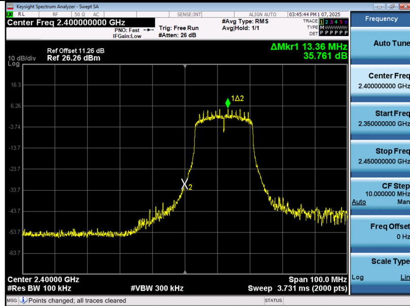
802.11n-CH 1
