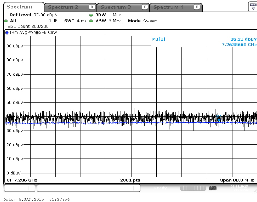
Radiated Spurious Emissions plot – Peak Result (802.11b_1 Mbps, Ch.1 3rd Harmonic, Y-V)
