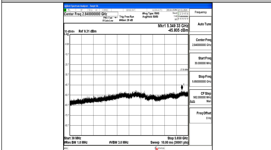
11AC80MIMO-Ant1-5775-30~5650-PASS
