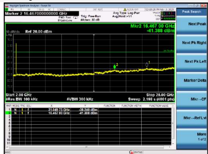
802.11g CHANNEL 6, SPURIOUS 2 GHz ~ 25 GHz
