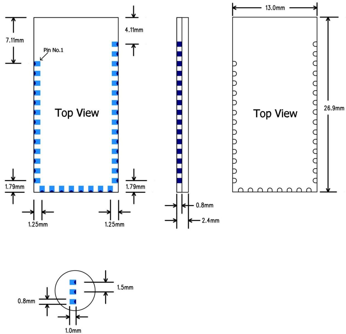
Figure 11: FSC-BT616 footprint
