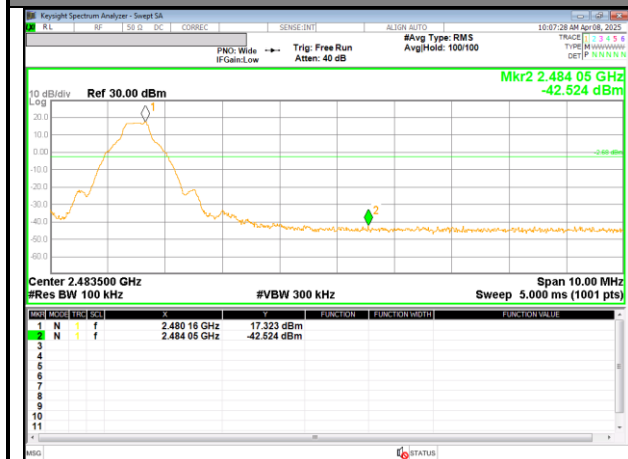
78 CHANNEL BANDEDGE
