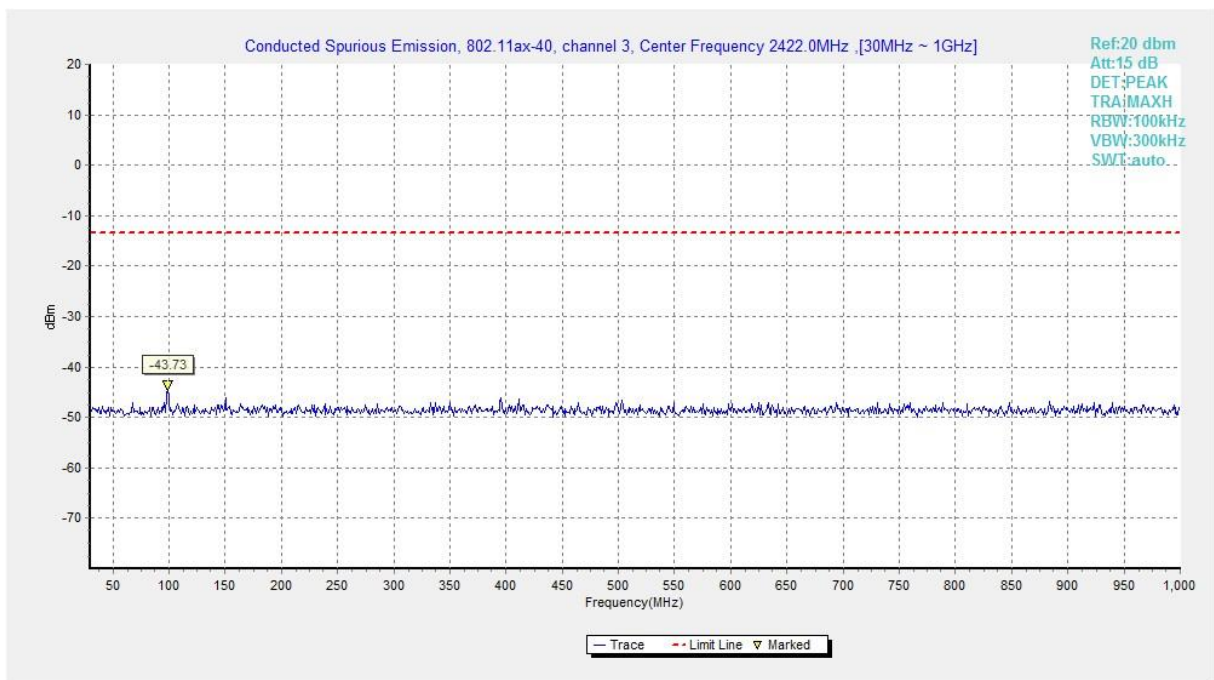
Fig.A.6.1.122 Transmitter Spurious Emission - Conducted (802.11ax-HE40, Ch3, 30 MHz-1 GHz)
