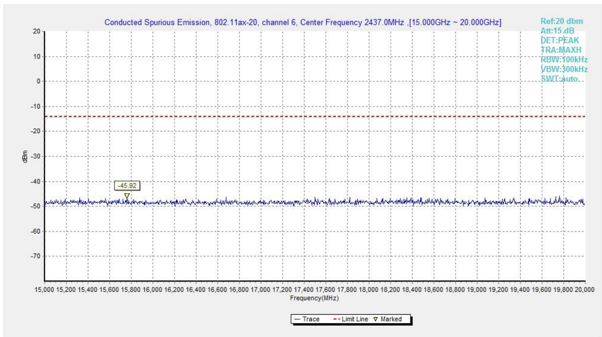
Fig.A.6.1.111 Transmitter Spurious Emission - Conducted (802.11ax-HE20, Ch6, 15 GHz-20 GHz)
