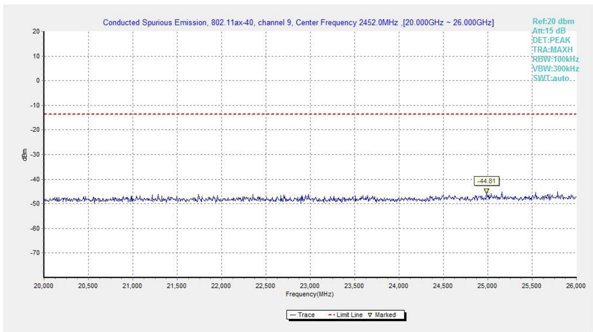
Fig.A.6.1.144 Transmitter Spurious Emission - Conducted (802.11ax-HE40, Ch9, 20 GHz-26 GHz)
