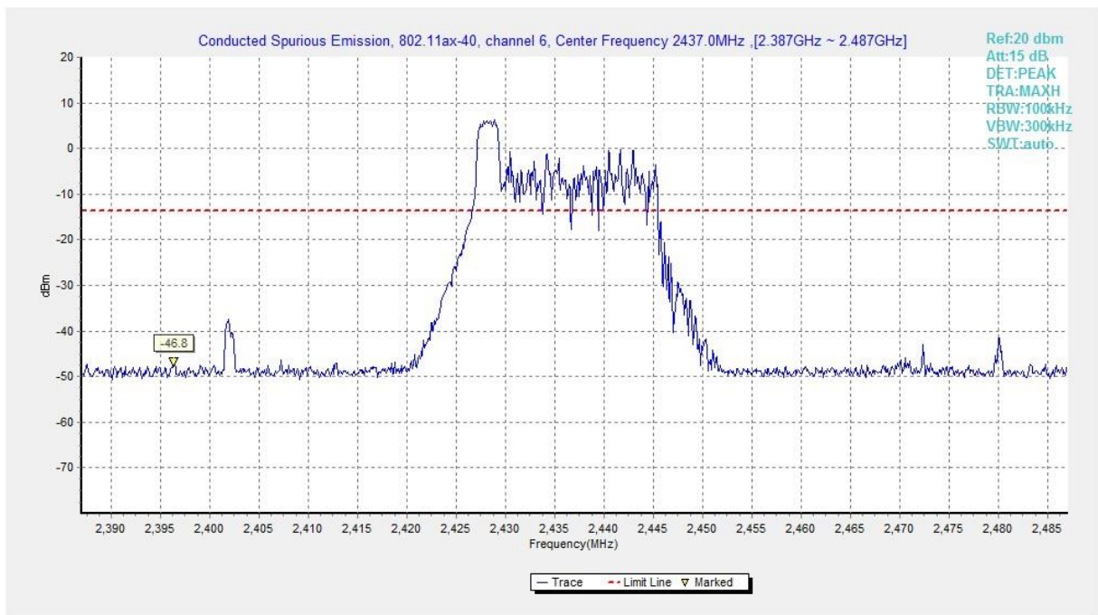
Fig.A.6.1.129 Transmitter Spurious Emission - Conducted (802.11ax-HE40, Ch6, Center Frequency)
