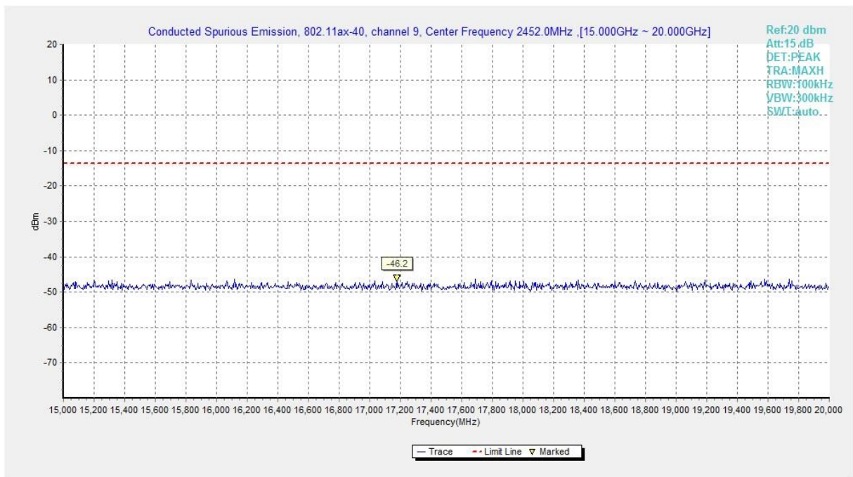
Fig.A.6.1.143 Transmitter Spurious Emission - Conducted (802.11ax-HE40, Ch9, 15 GHz-20 GHz)
