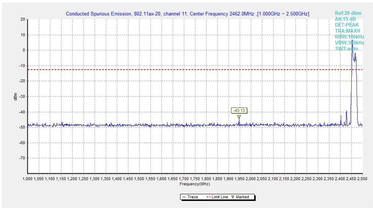
Fig.A.6.1.115 Transmitter Spurious Emission - Conducted (802.11ax-HE20, Ch11, 1 GHz-2.5 GHz)
