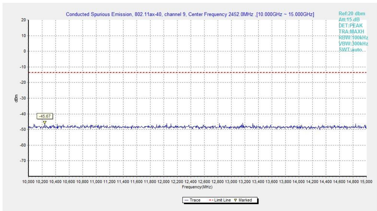
Fig.A.6.1.142 Transmitter Spurious Emission - Conducted (802.11ax-HE40, Ch9, 10 GHz-15 GHz)
