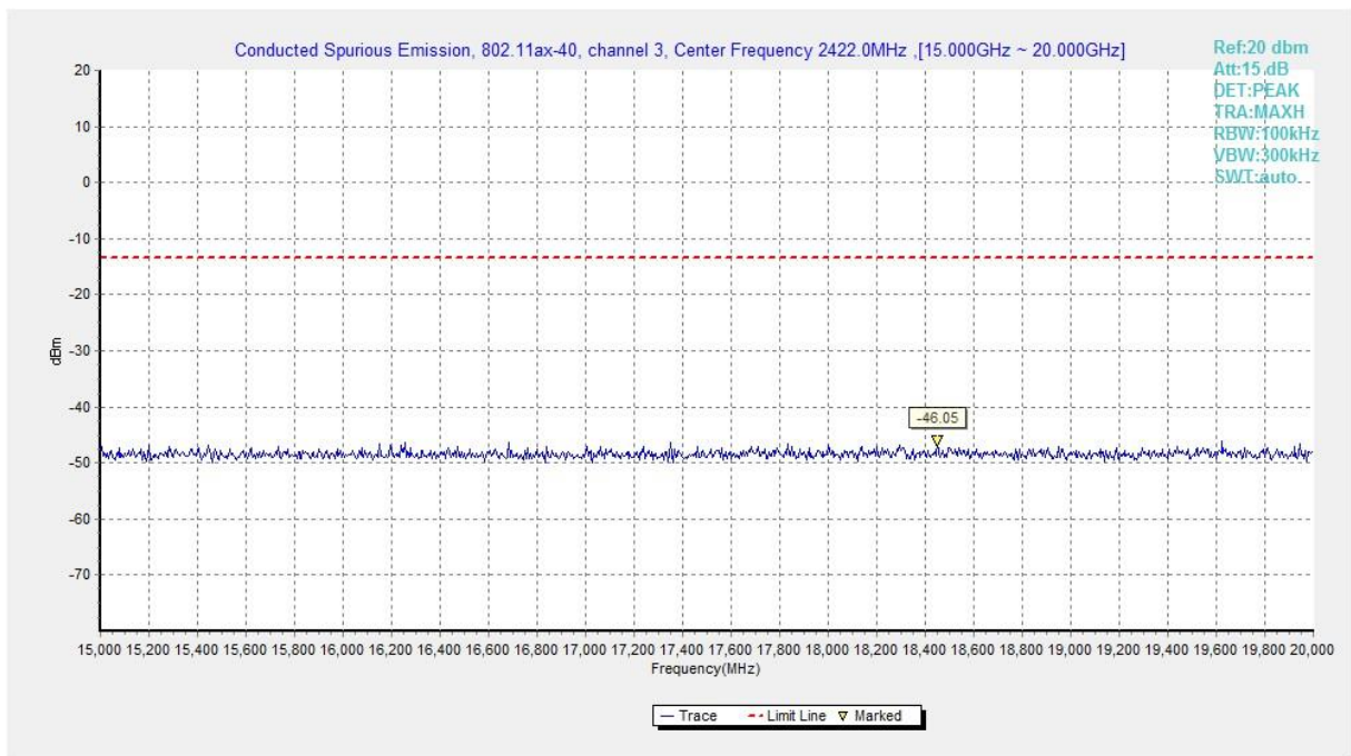
Fig.A.6.1.127 Transmitter Spurious Emission - Conducted (802.11ax-HE40, Ch3, 15 GHz-20 GHz)
