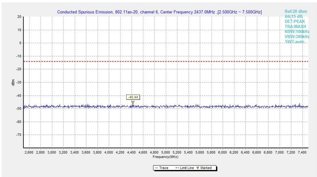
Fig.A.6.1.108 Transmitter Spurious Emission - Conducted (802.11ax-HE20, Ch6, 2.5 GHz-7.5 GHz)
