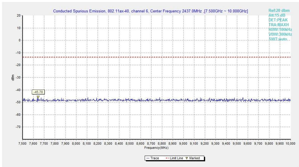
Fig.A.6.1.133 Transmitter Spurious Emission - Conducted (802.11ax-HE40, Ch6, 7.5 GHz-10 GHz)
