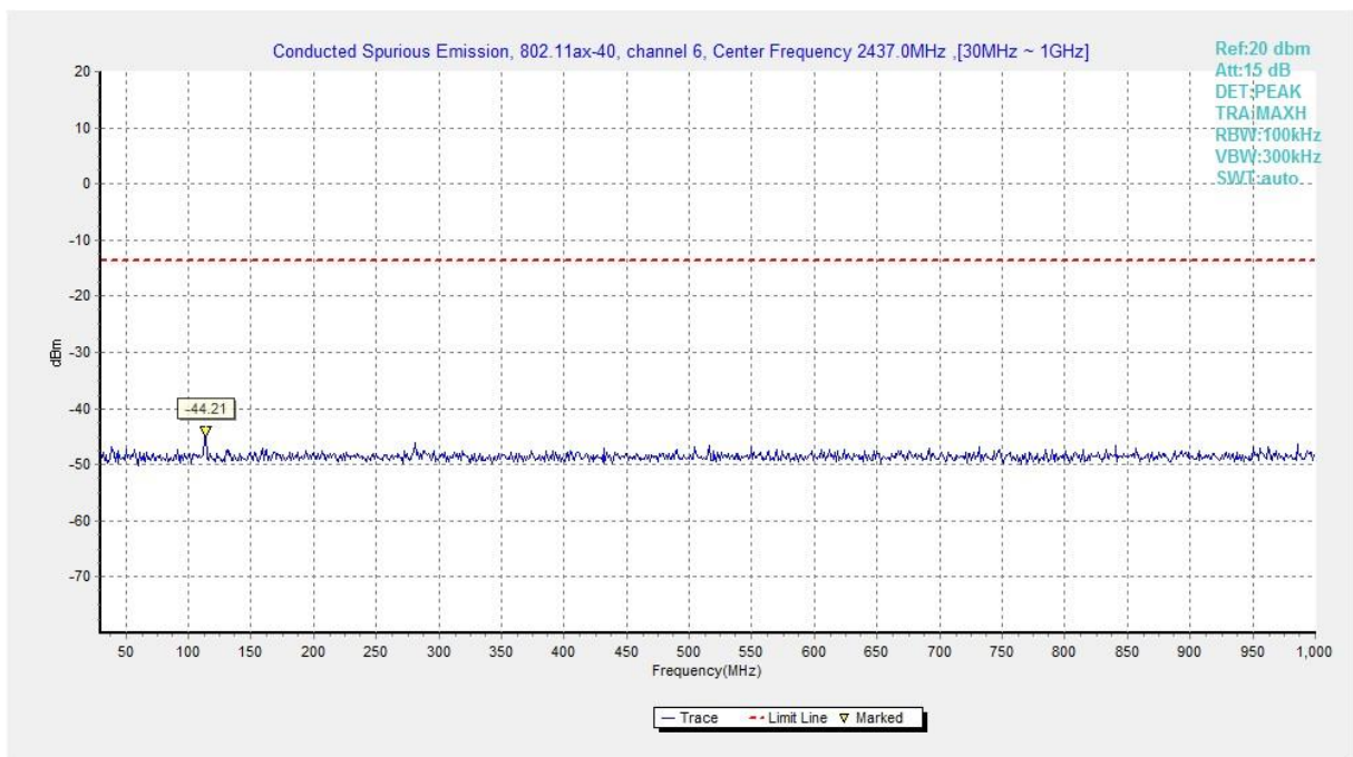
Fig.A.6.1.130 Transmitter Spurious Emission - Conducted (802.11ax-HE40, Ch6, 30 MHz-1 GHz)
