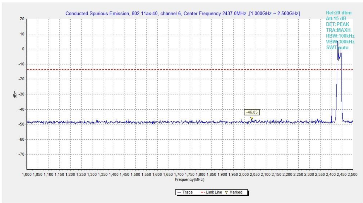
Fig.A.6.1.131 Transmitter Spurious Emission - Conducted (802.11ax-HE40, Ch6, 1 GHz-2.5 GHz)
