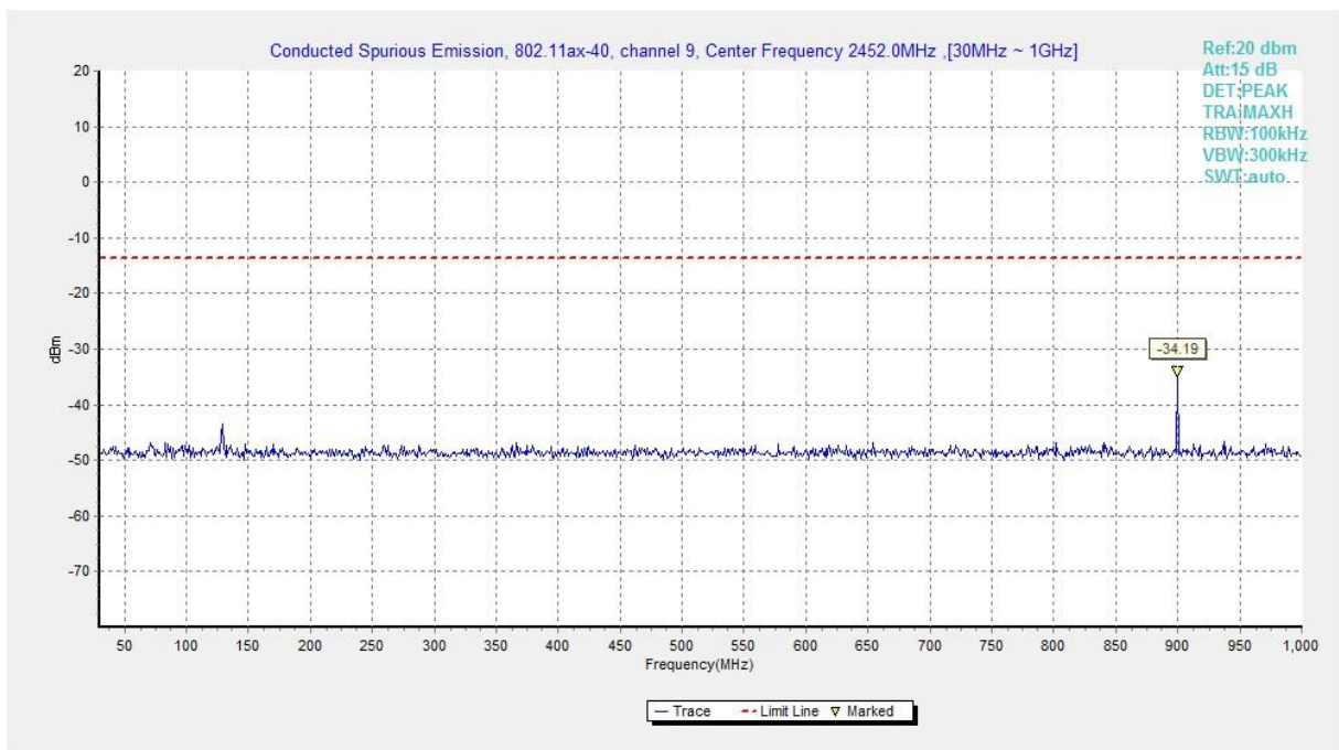
Fig.A.6.1.138 Transmitter Spurious Emission - Conducted (802.11ax-HE40, Ch9, 30 MHz-1 GHz)
