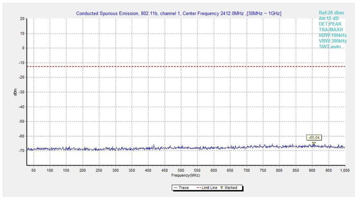
Fig.A.6.1.146 Transmitter Spurious Emission - Conducted (802.11b, Ch1, 30 MHz-1 GHz)
