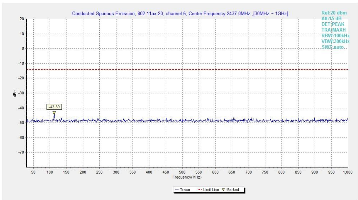
Fig.A.6.1.106 Transmitter Spurious Emission - Conducted (802.11ax-HE20, Ch6, 30 MHz-1 GHz)
