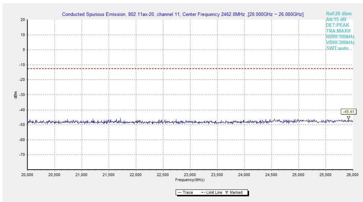
Fig.A.6.1.120 Transmitter Spurious Emission - Conducted (802.11ax-HE20, Ch11, 20 GHz-26 GHz)
