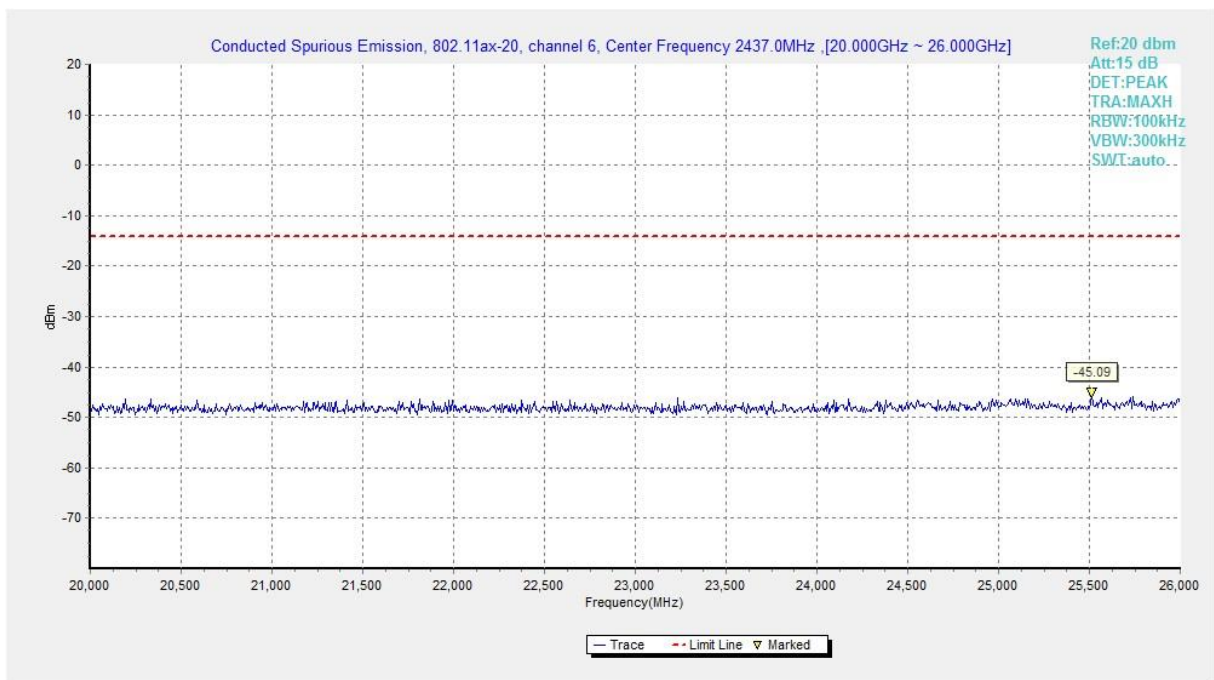
Fig.A.6.1.112 Transmitter Spurious Emission - Conducted (802.11ax-HE20, Ch6, 20 GHz-26 GHz)
