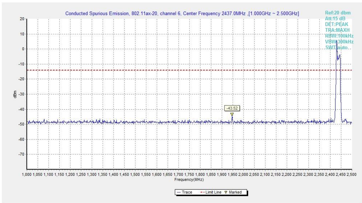
Fig.A.6.1.107 Transmitter Spurious Emission - Conducted (802.11ax-HE20, Ch6, 1 GHz-2.5 GHz)
