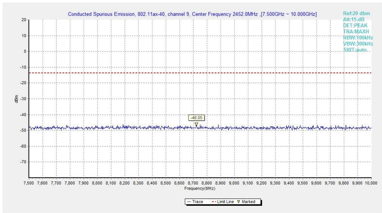
Fig.A.6.1.141 Transmitter Spurious Emission - Conducted (802.11ax-HE40, Ch9, 7.5 GHz-10 GHz)
