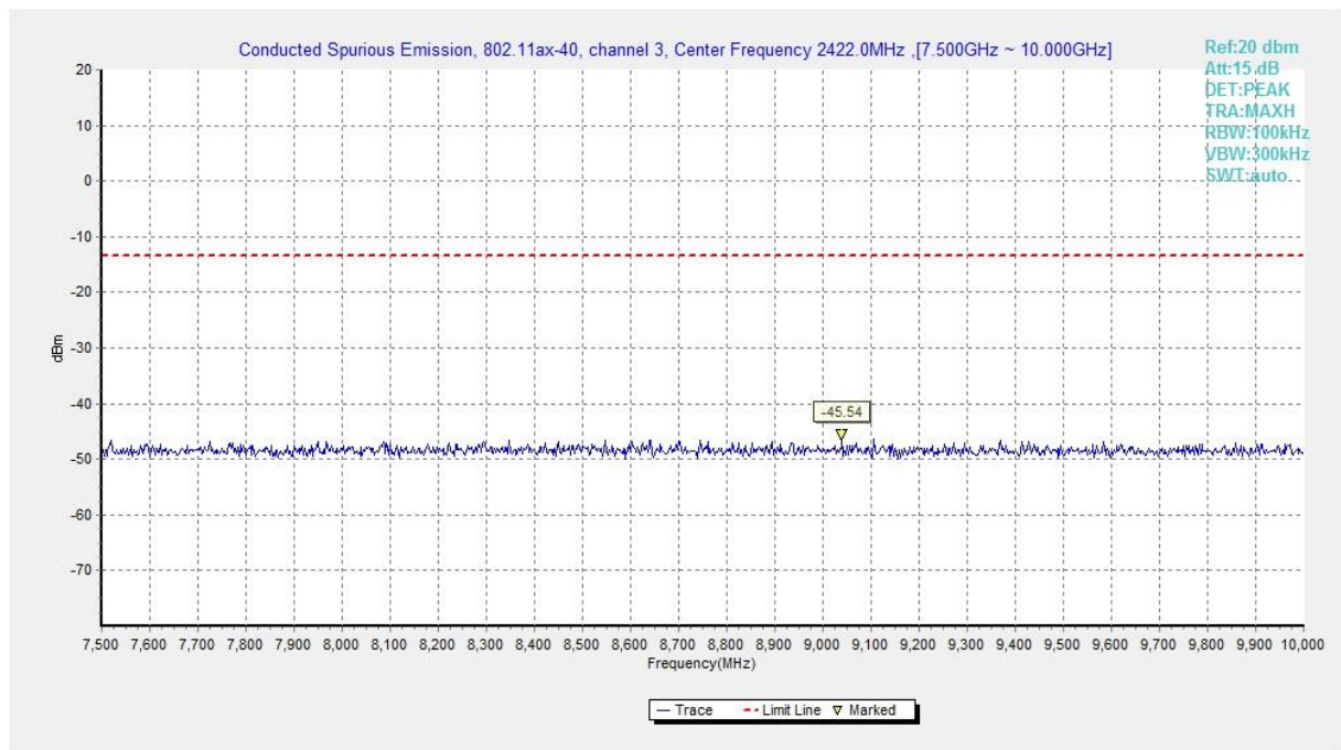
Fig.A.6.1.125 Transmitter Spurious Emission - Conducted (802.11ax-HE40, Ch3, 7.5 GHz-10 GHz)
