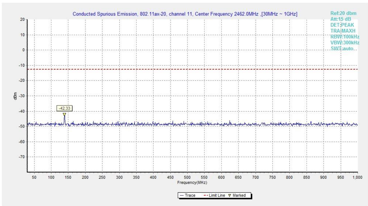
Fig.A.6.1.114 Transmitter Spurious Emission - Conducted (802.11ax-HE20, Ch11, 30 MHz-1 GHz)
