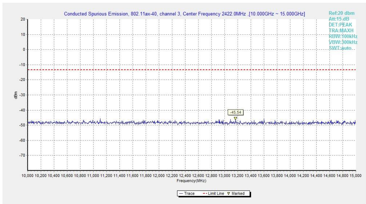
Fig.A.6.1.126 Transmitter Spurious Emission - Conducted (802.11ax-HE40, Ch3, 10 GHz-15 GHz)
