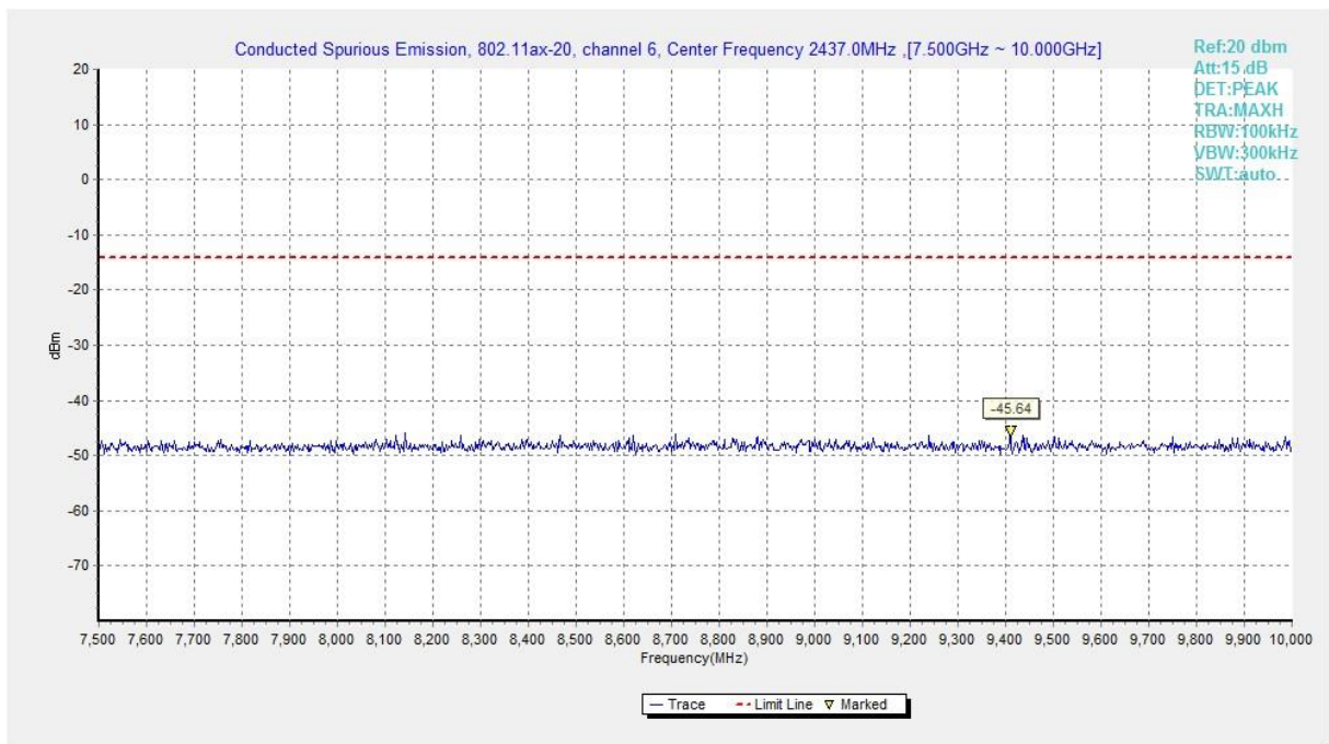
Fig.A.6.1.109 Transmitter Spurious Emission - Conducted (802.11ax-HE20, Ch6, 7.5 GHz-10 GHz)
