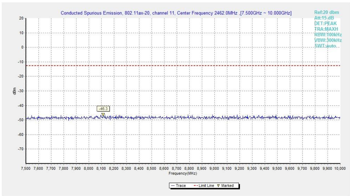
Fig.A.6.1.117 Transmitter Spurious Emission - Conducted (802.11ax-HE20, Ch11, 7.5 GHz-10 GHz)
