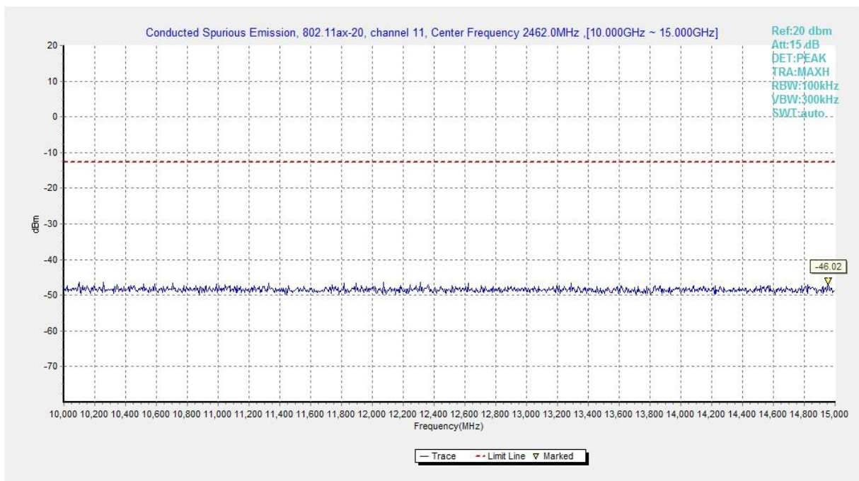
Fig.A.6.1.118 Transmitter Spurious Emission - Conducted (802.11ax-HE20, Ch11, 10 GHz-15 GHz)
