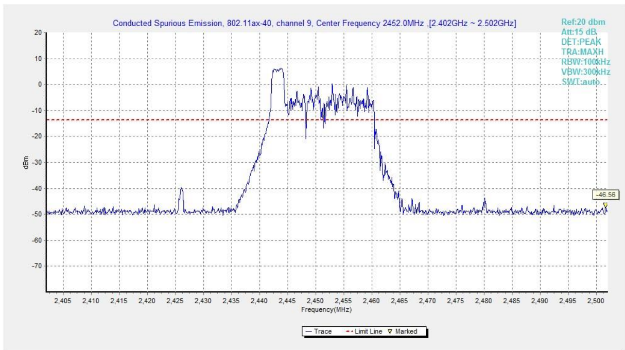
Fig.A.6.1.137 Transmitter Spurious Emission - Conducted (802.11ax-HE40, Ch9, Center Frequency)
