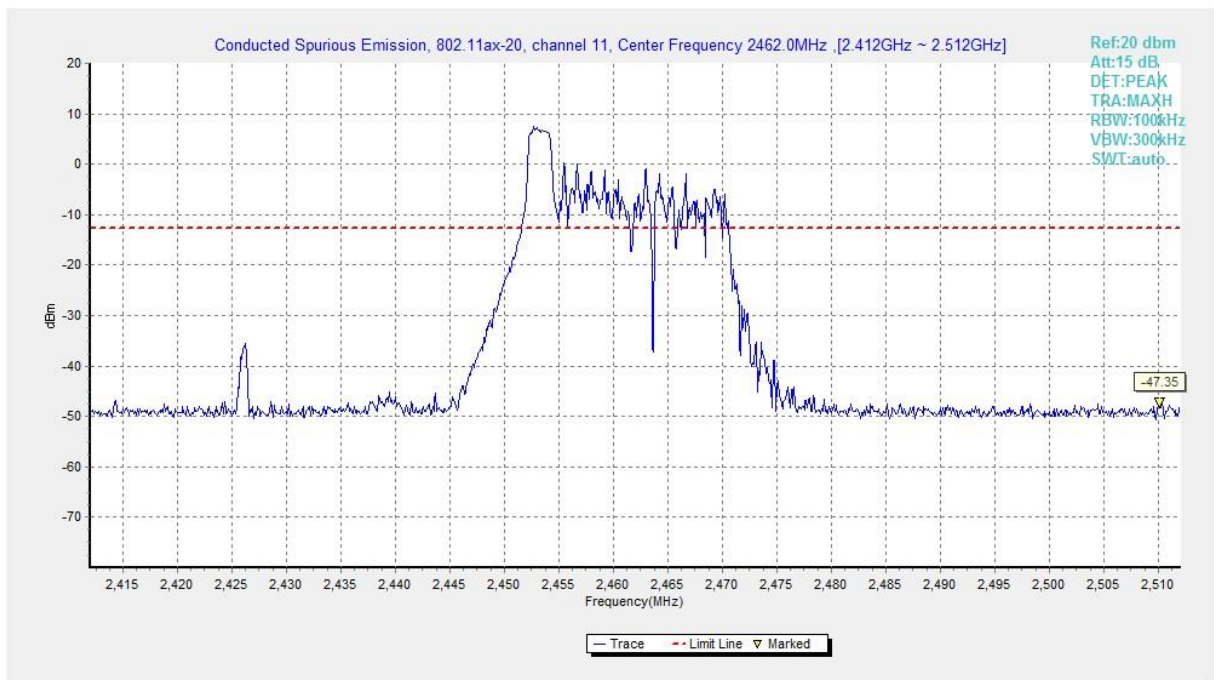
Fig.A.6.1.113 Transmitter Spurious Emission - Conducted (802.11ax-HE20, Ch11, Center Frequency)
