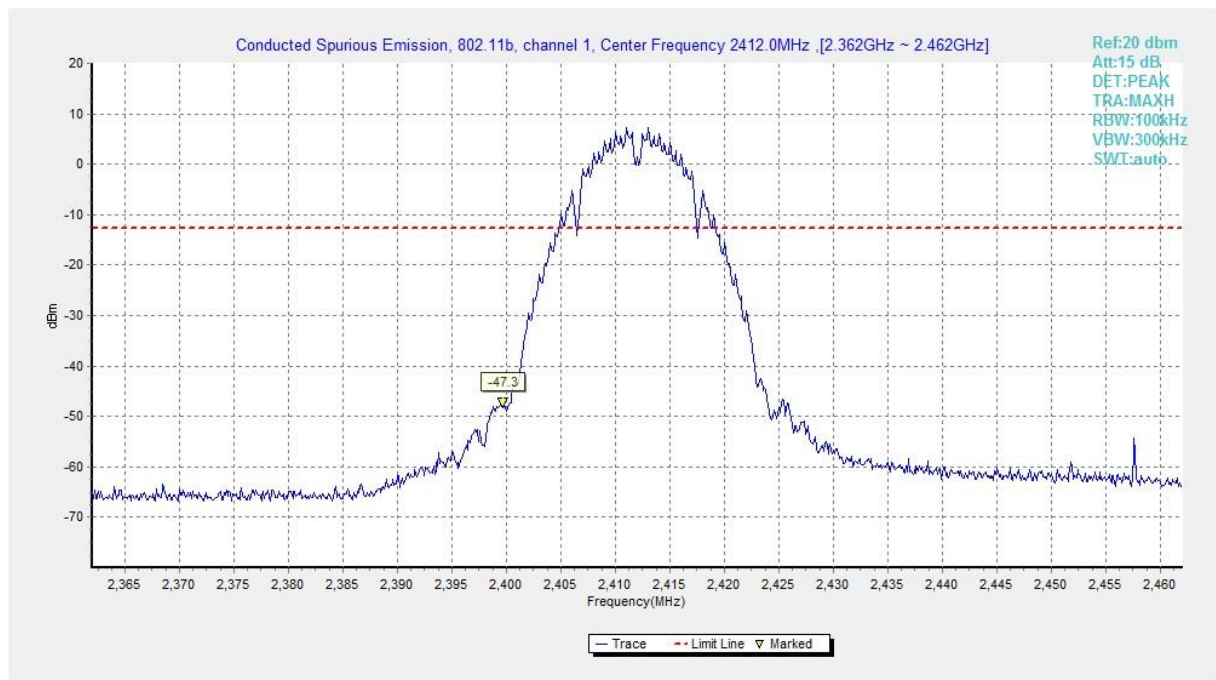
Fig.A.6.1.145 Transmitter Spurious Emission - Conducted (802.11b, Ch1, Center Frequency)
