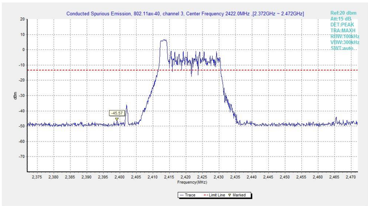
Fig.A.6.1.121 Transmitter Spurious Emission - Conducted (802.11ax-HE40, Ch3, Center Frequency)
