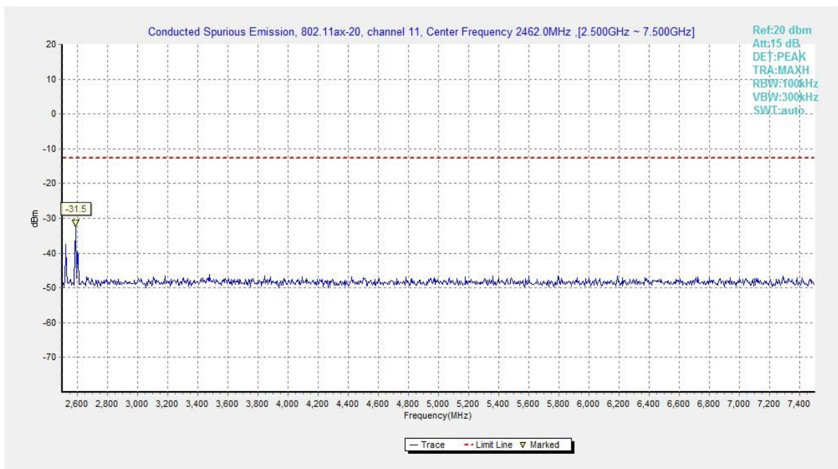
Fig.A.6.1.116 Transmitter Spurious Emission - Conducted (802.11ax-HE20, Ch11, 2.5 GHz-7.5 GHz)
