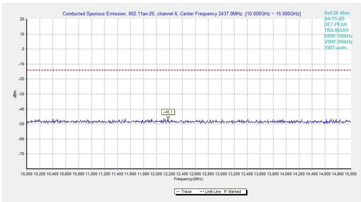
Fig.A.6.1.110 Transmitter Spurious Emission - Conducted (802.11ax-HE20, Ch6, 10 GHz-15 GHz)
