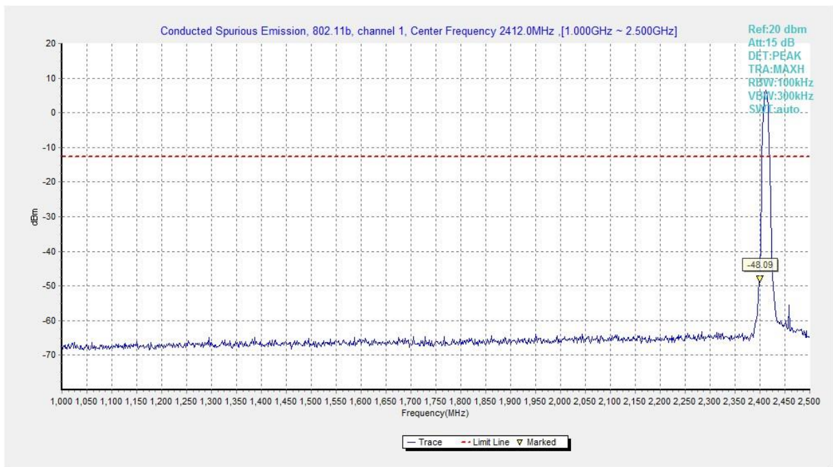
Fig.A.6.1.147 Transmitter Spurious Emission - Conducted (802.11b, Ch1, 1 GHz-2.5 GHz)
