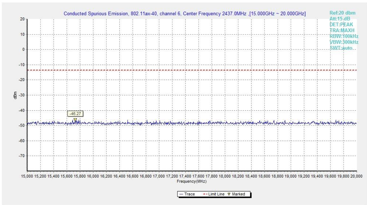
Fig.A.6.1.135 Transmitter Spurious Emission - Conducted (802.11ax-HE40, Ch6, 15 GHz-20 GHz)
