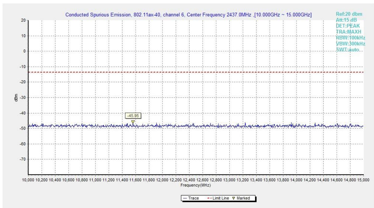
Fig.A.6.1.134 Transmitter Spurious Emission - Conducted (802.11ax-HE40, Ch6, 10 GHz-15 GHz)
