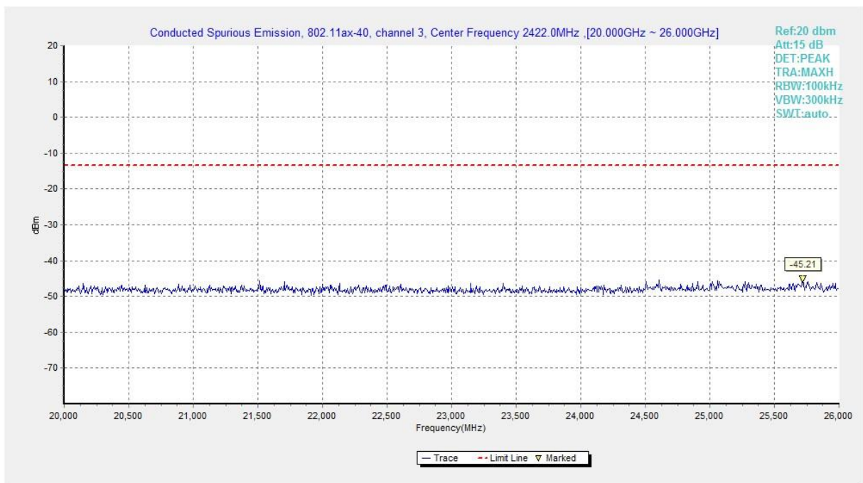
Fig.A.6.1.128 Transmitter Spurious Emission - Conducted (802.11ax-HE40, Ch3, 20 GHz-26 GHz)
