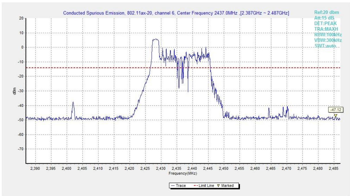
Fig.A.6.1.105 Transmitter Spurious Emission - Conducted (802.11ax-HE20, Ch6, Center Frequency)
