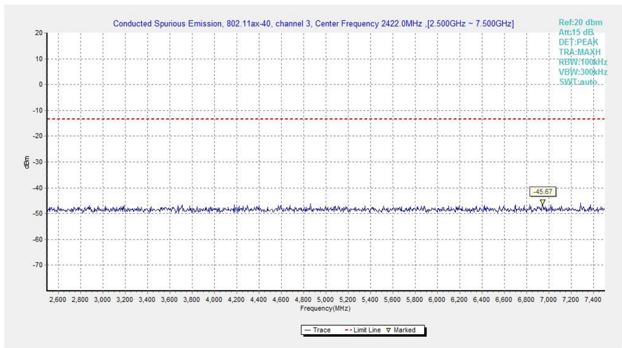
Fig.A.6.1.124 Transmitter Spurious Emission - Conducted (802.11ax-HE40, Ch3, 2.5 GHz-7.5 GHz)
