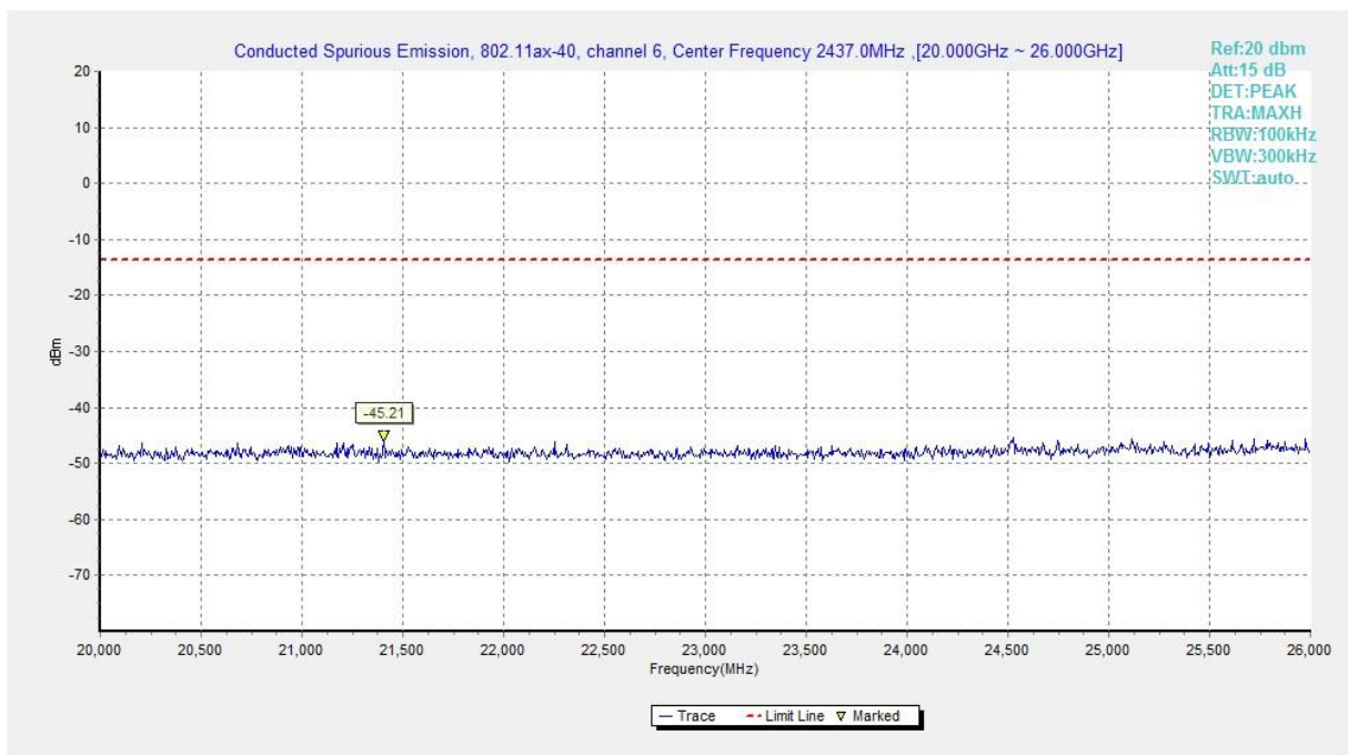
Fig.A.6.1.136 Transmitter Spurious Emission - Conducted (802.11ax-HE40, Ch6, 20 GHz-26 GHz)
