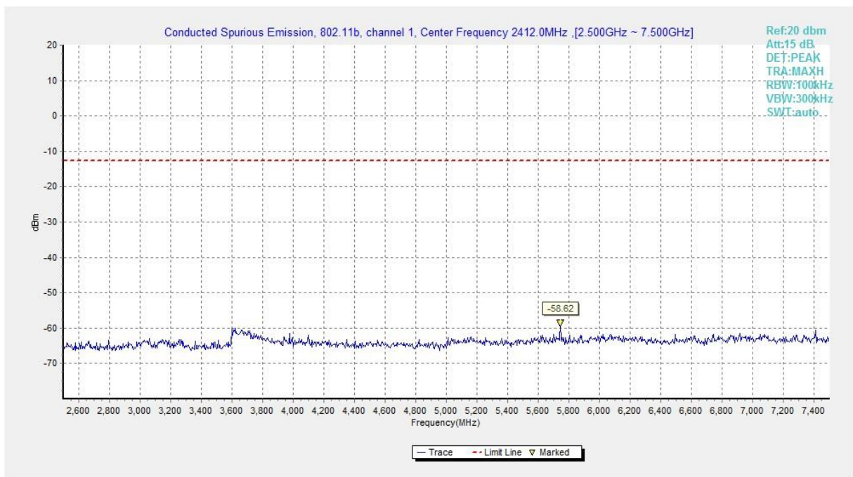
Fig.A.6.1.148 Transmitter Spurious Emission - Conducted (802.11b, Ch1, 2.5 GHz-7.5 GHz)
