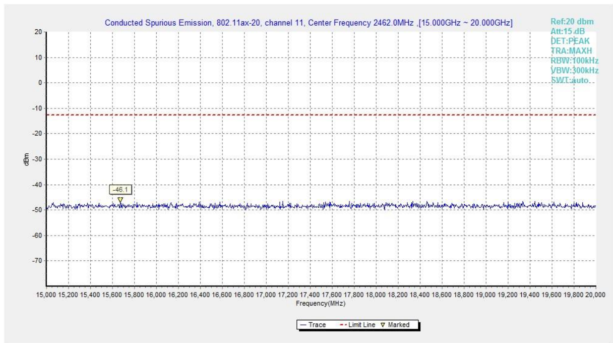
Fig.A.6.1.119 Transmitter Spurious Emission - Conducted (802.11ax-HE20, Ch11, 15 GHz-20 GHz)
