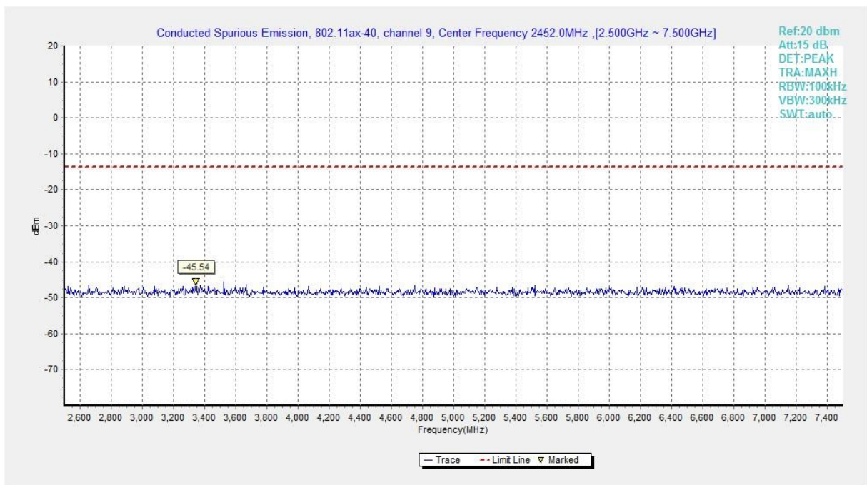
Fig.A.6.1.140 Transmitter Spurious Emission - Conducted (802.11ax-HE40, Ch9, 2.5 GHz-7.5 GHz)
