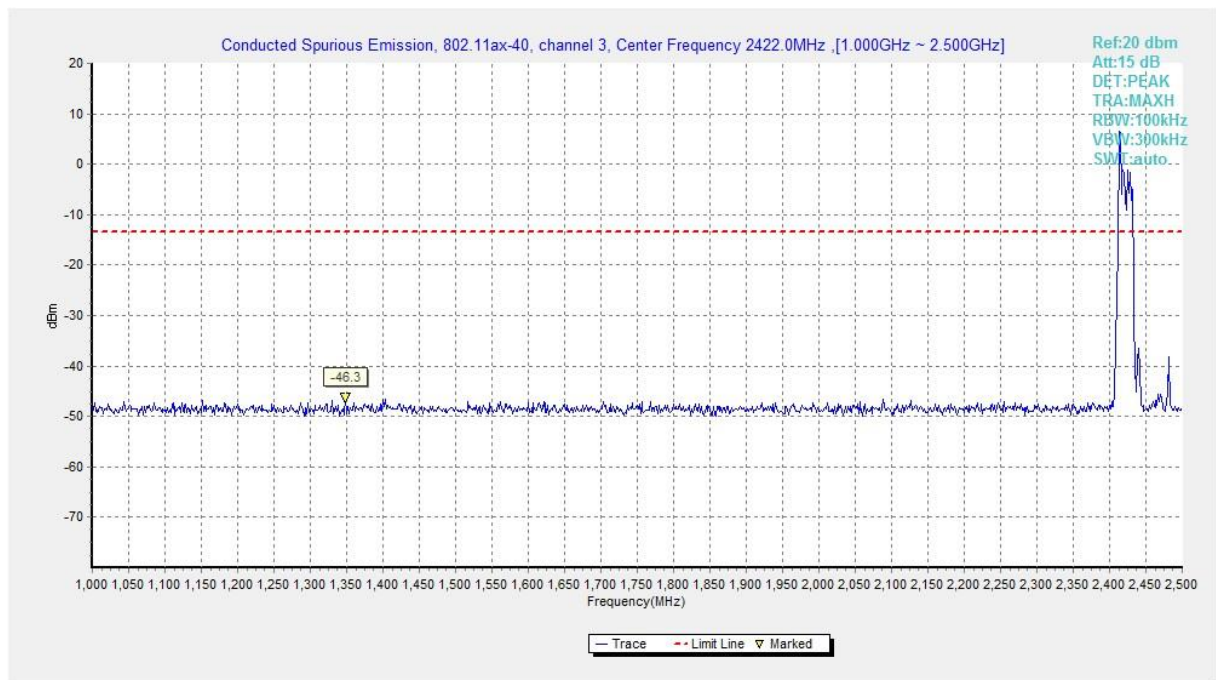
Fig.A.6.1.123 Transmitter Spurious Emission - Conducted (802.11ax-HE40, Ch3, 1 GHz-2.5 GHz)
