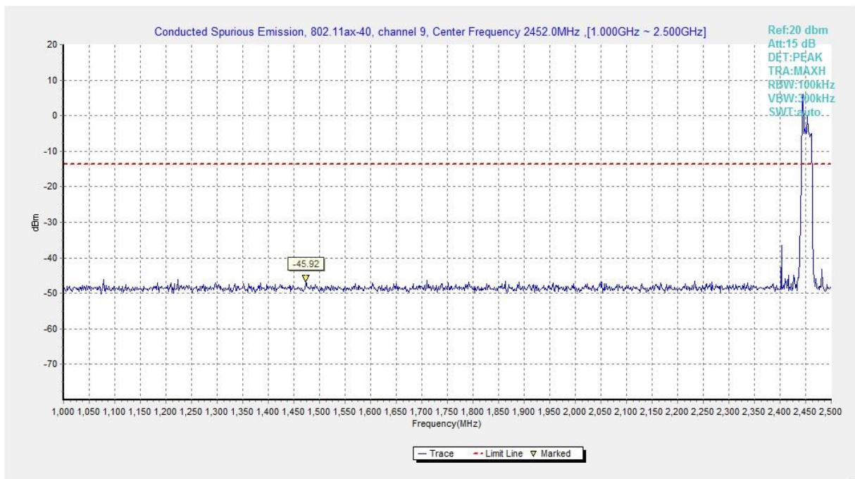
Fig.A.6.1.139 Transmitter Spurious Emission - Conducted (802.11ax-HE40, Ch9, 1 GHz-2.5 GHz)
