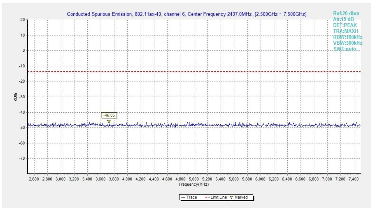
Fig.A.6.1.132 Transmitter Spurious Emission - Conducted (802.11ax-HE40, Ch6, 2.5 GHz-7.5 GHz)
