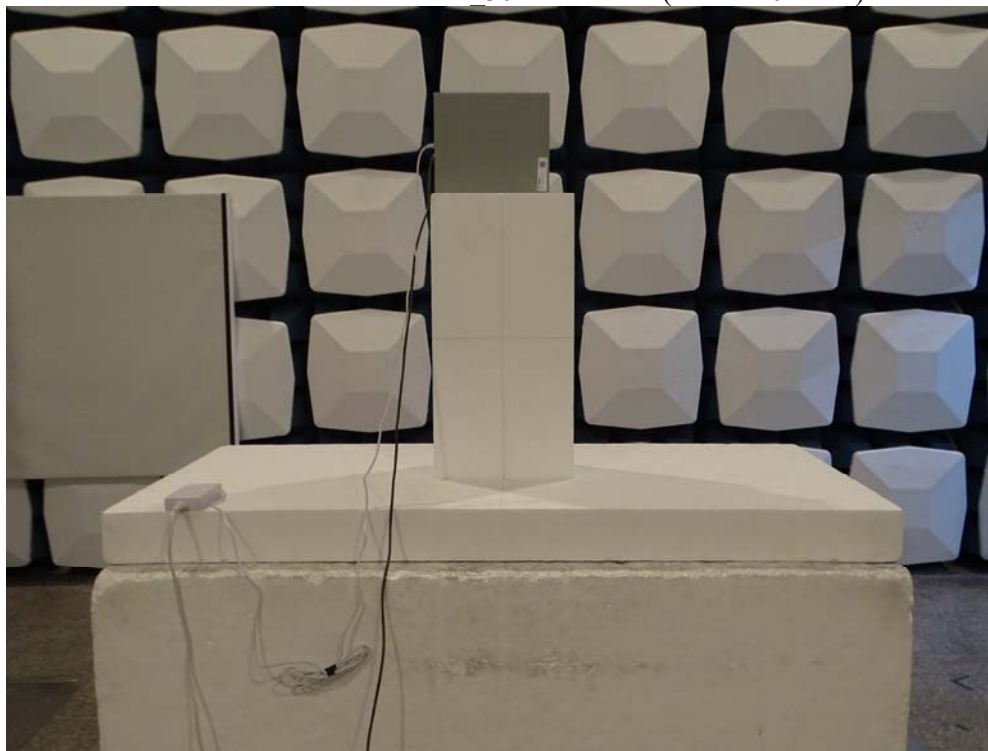
Back View of Radiated Test 30MHz-1GHz (ADP-120VH D)
