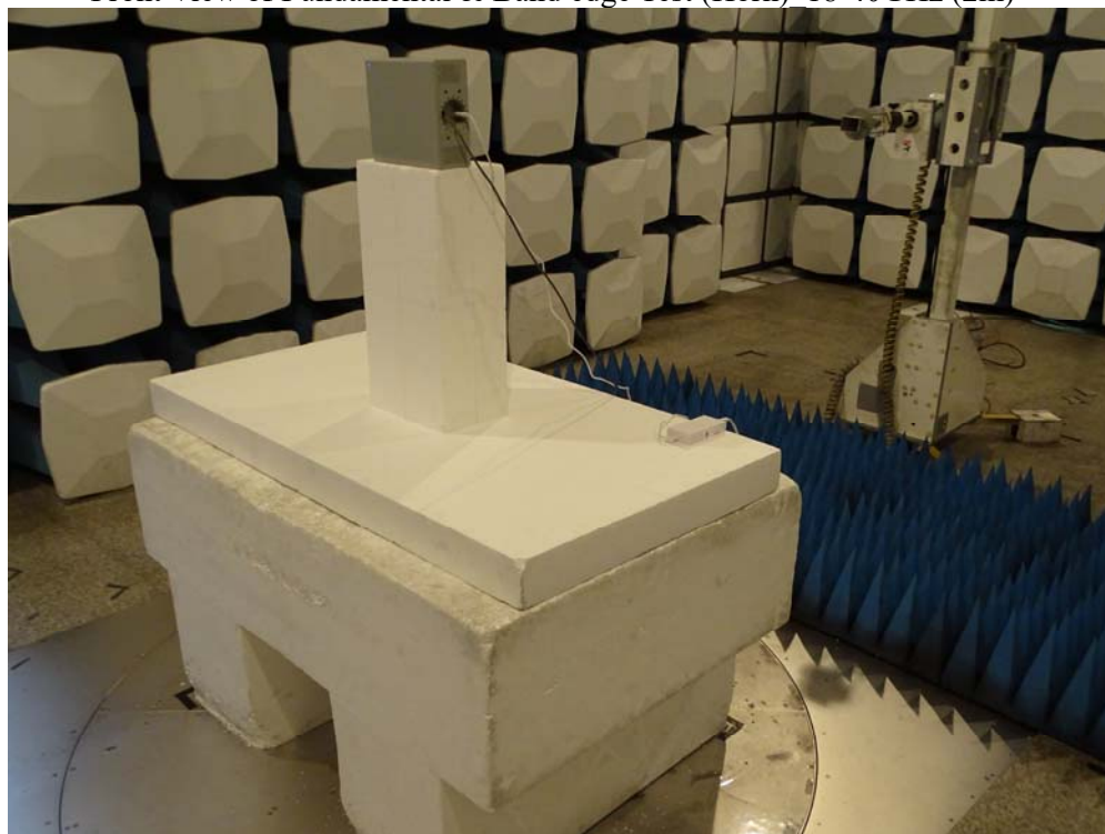
Front View of Fundamental & Band edge Test (Horn) 18-40GHz (2m)
