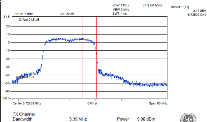
802.11n (HT40) CDD / Chain 3 : CH 142 (U-NII-3)
