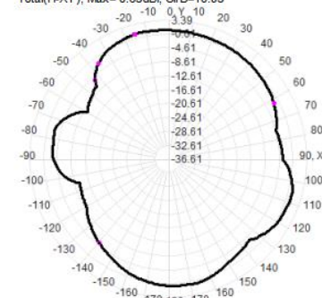
Total(H+XY), Max= 0.65dBi, CirD=10.85
