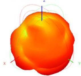
2415.0MHz H+V, Eff: 54.1%
