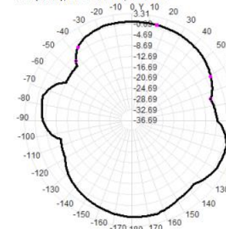
Total(H-XY), Max= 0.19dBi, CirD=9.65
