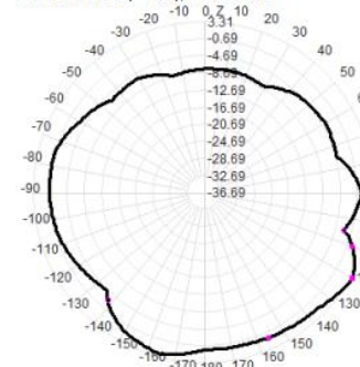
2460.0MHz Total(E2-YZ), Max= 3.31dBi
