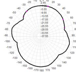
Total(H-XY), Max= -0.77dBi, CirD=8.85
