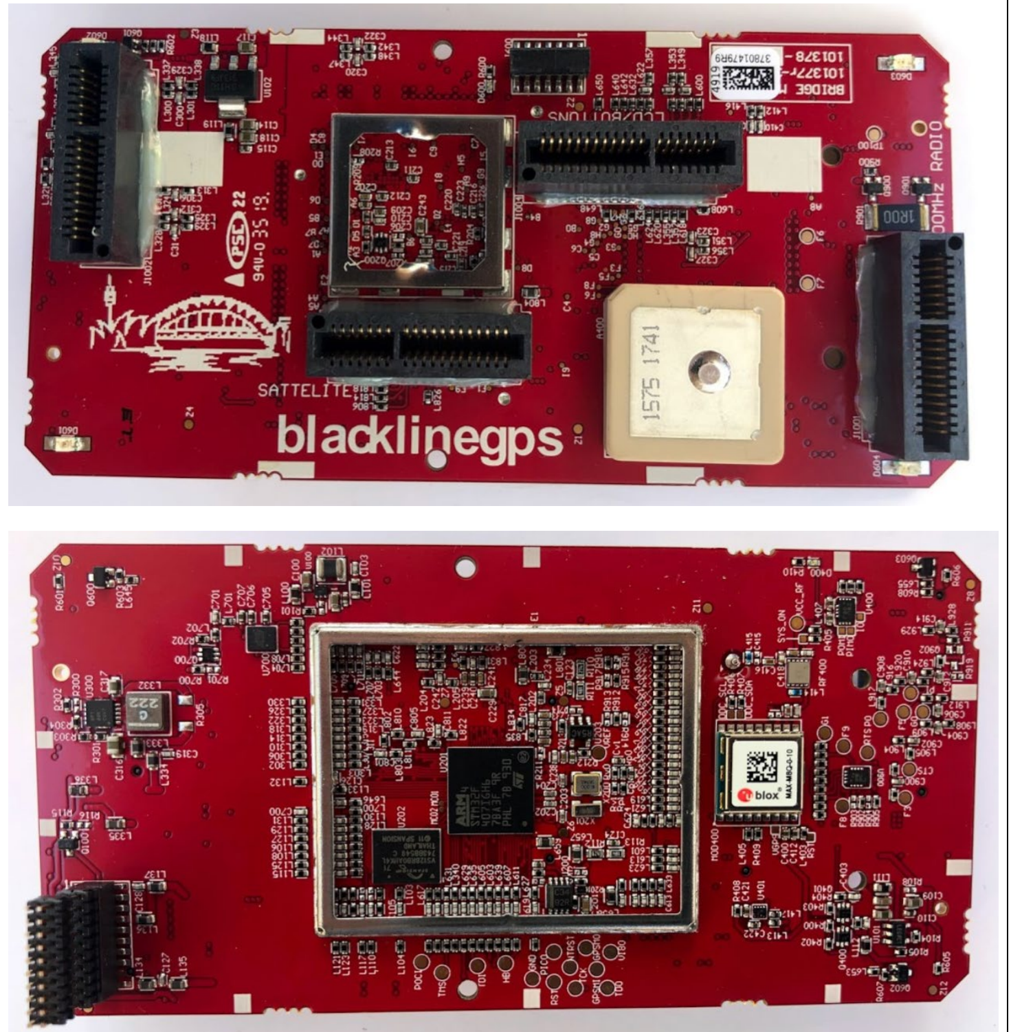
Main PCB
