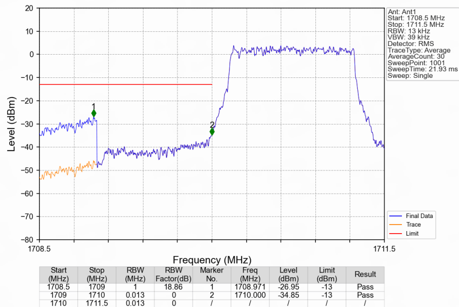
Band4_1.4MHz_QPSK_LCH_1710.7MHz_RB_6_0_NTNV
