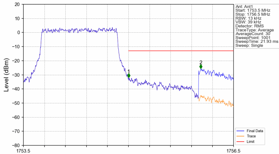
Band4_1.4MHz_QPSK_HCH_1754.3MHz_RB_6_0_NTNV
