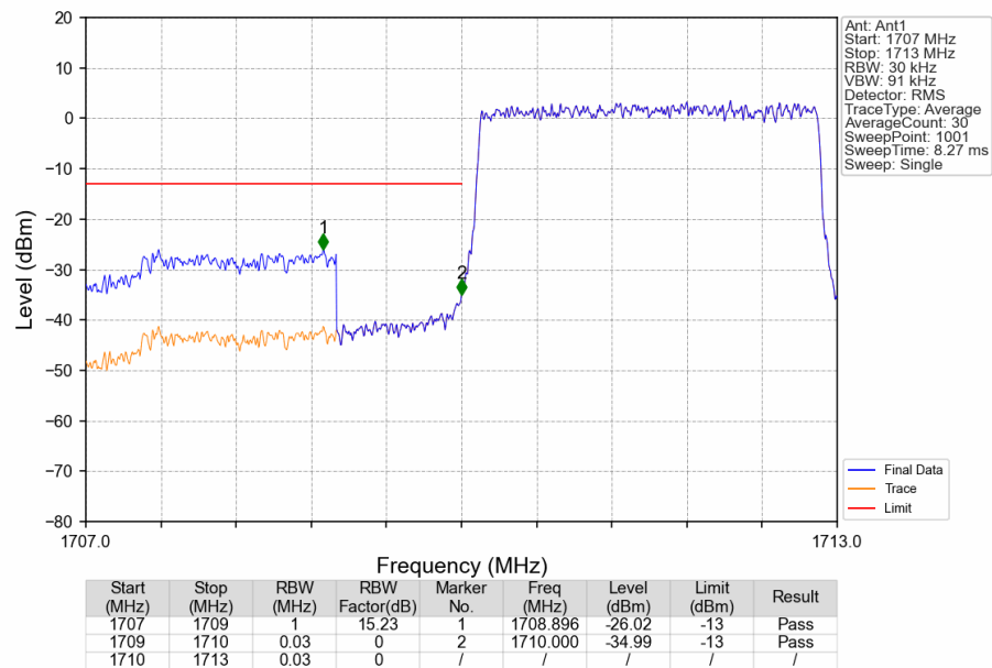
Band4_3MHz_QPSK_LCH_1711.5MHz_RB_15_0_NTNV
