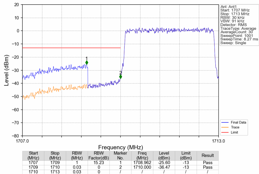
Band4_3MHz_16QAM_LCH_1711.5MHz_RB_15_0_NTNV
