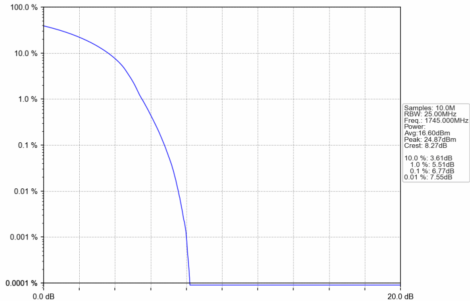
Band4_20MHz_16QAM_HCH_1745MHz_RB_100_0_NTNV
