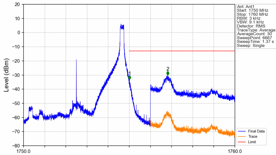
Band4_5MHz_QPSK_HCH_1752.5MHz_RB_1_24_NTNV
