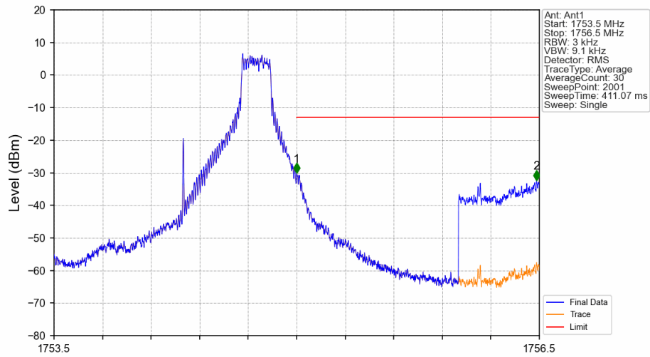
Band4_1.4MHz_QPSK_HCH_1754.3MHz_RB_1_5_NTNV
