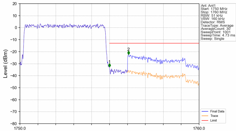
Band4_5MHz_QPSK_HCH_1752.5MHz_RB_25_0_NTNV
