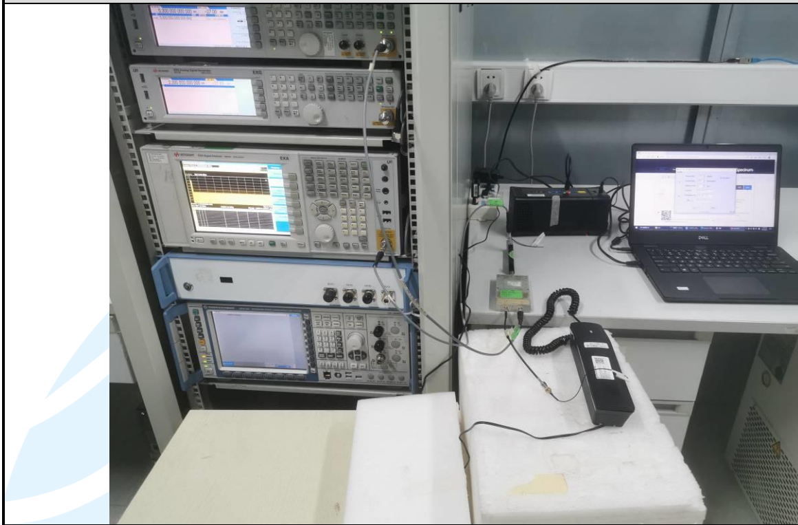
DFS Test Setup
