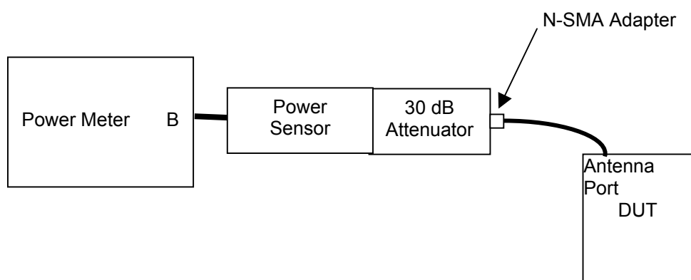
Figure C-1 - Setup Drawing
