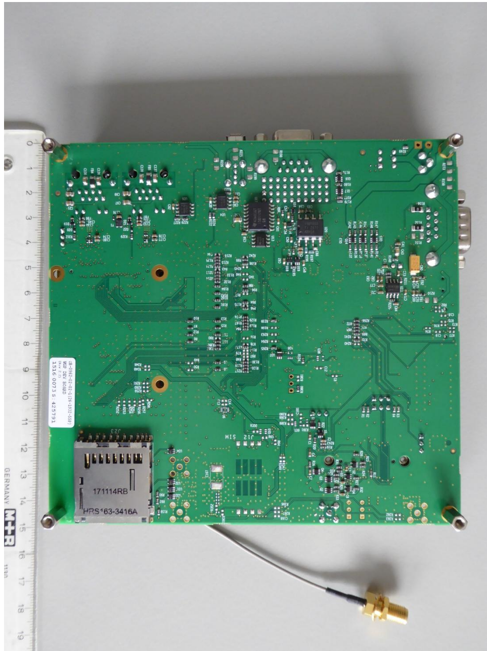
160912_DFS5.JPG: Carrier board, bottom view
