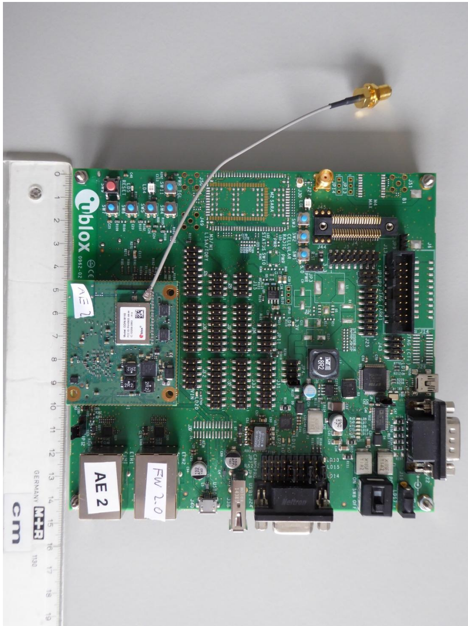
160912_DFS4.JPG: ODIN-W160, mouted on carrier board, top view
