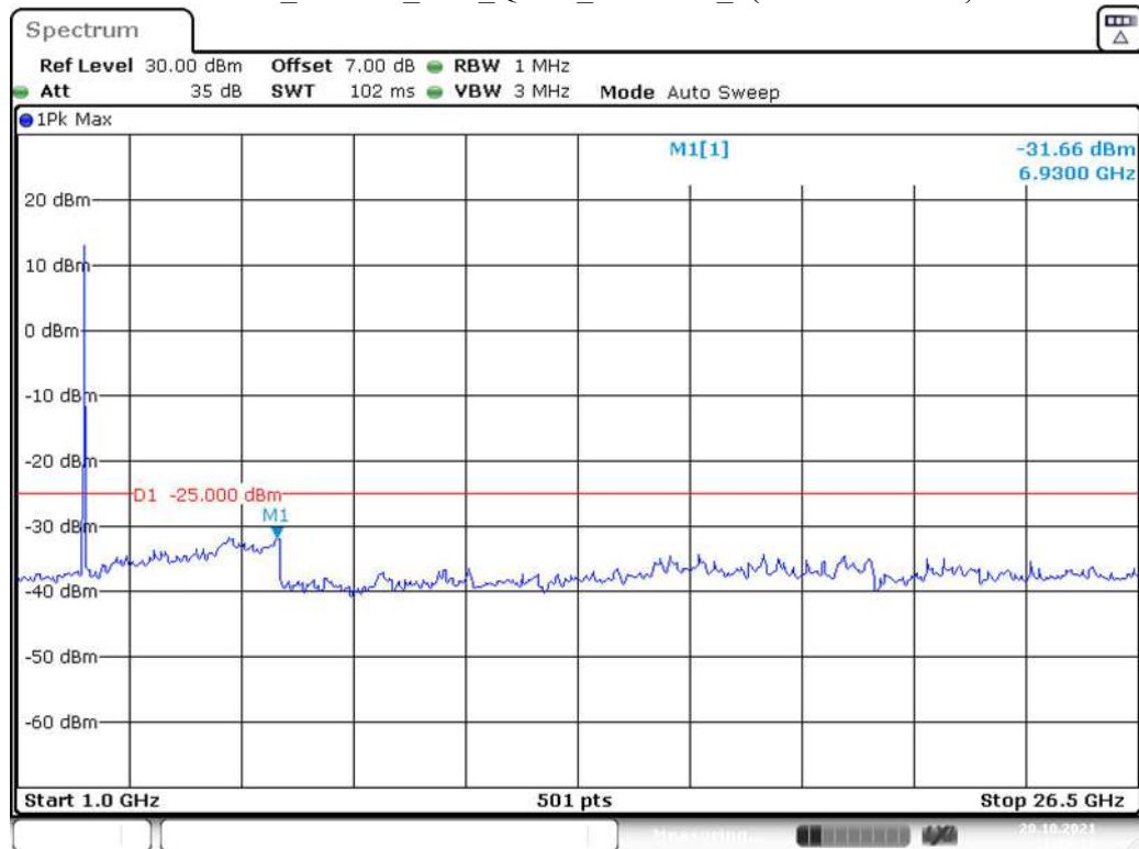
Band 41_20 MHz_Low_QPSK_RB100#0_2(1GHz-26.5GHz)
