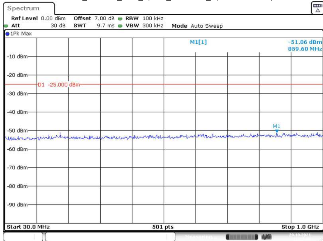
Band 41_20 MHz_Low_QPSK_RB100#0_1(30MHz-1GHz)
