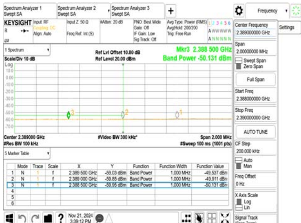
802.11ax_40MHz_2437MHz_RU242_62_R
