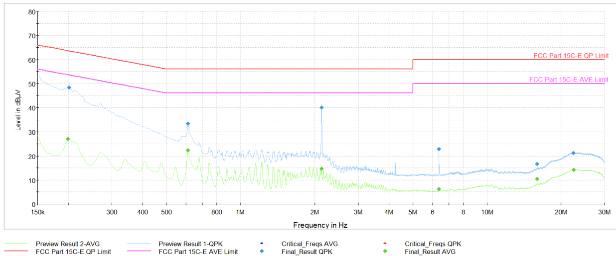
Plot 7-35. AC Line Conducted Plot with Bluetooth LE (L1, 1Mbps, Ch.19 with host PC via USB-C cable with wire charger)
