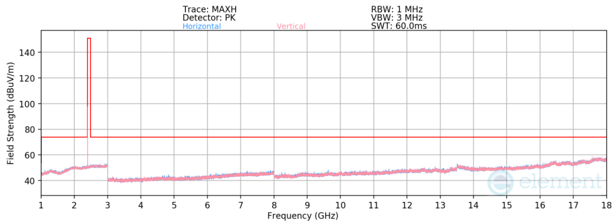
Plot 7-23. Radiated Spurious Emissions 1-18GHz (1Mbps – Ch. 0)
