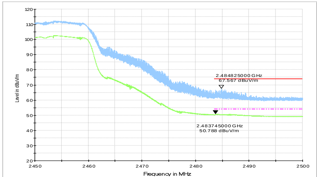
Fig.A.6.2.5 Transmitter Spurious Emission - Radiated (Power): 802.11g, ch9, 2.45 GHz - 2.50GHz
