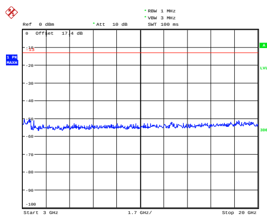
eMTC Band 2 3MHz CH-High 3GHz~20GHz
