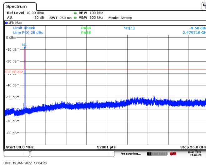
Figure 8.6-3: Conducted spurious emissions Tx on high channel
