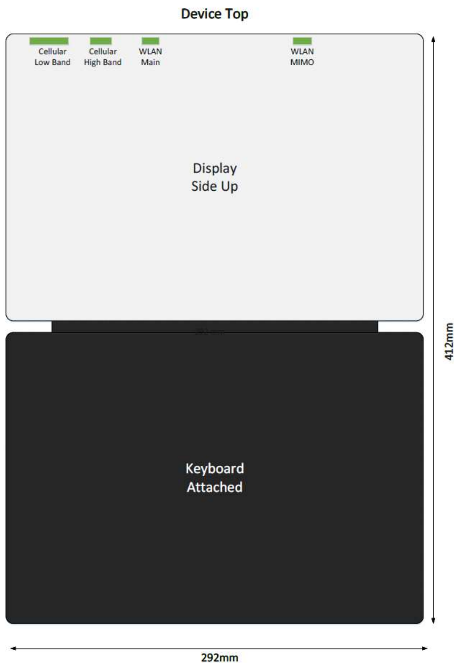
Fig. 2 - Device Dimensions with Keyboard Attached
