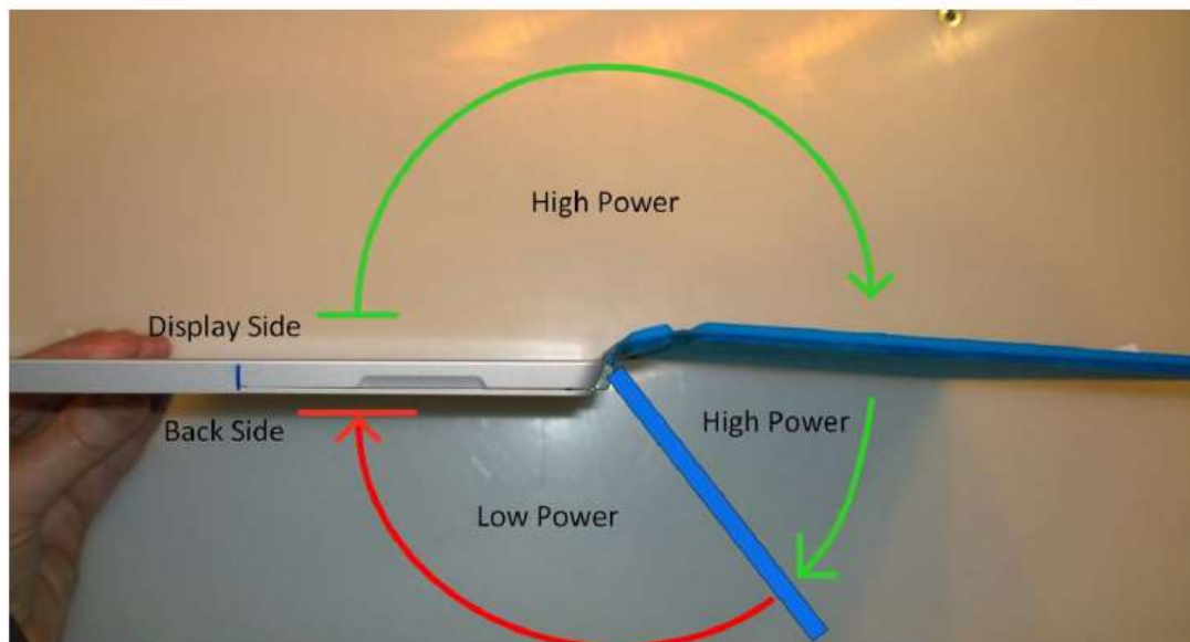
Fig. 3 – WLAN Output Power Relative to Keyboard Angle
