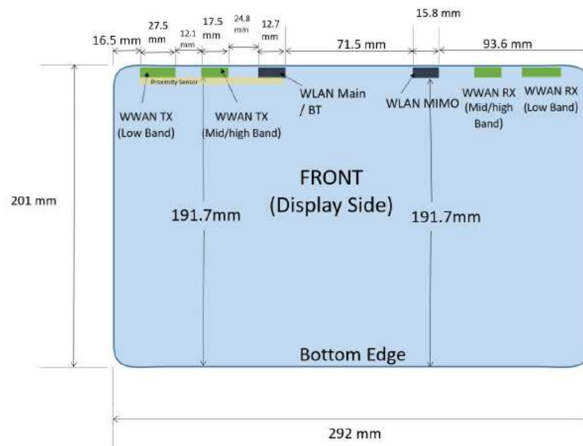
Fig. 1 - Tablet Dimensions and Antenna Locations
