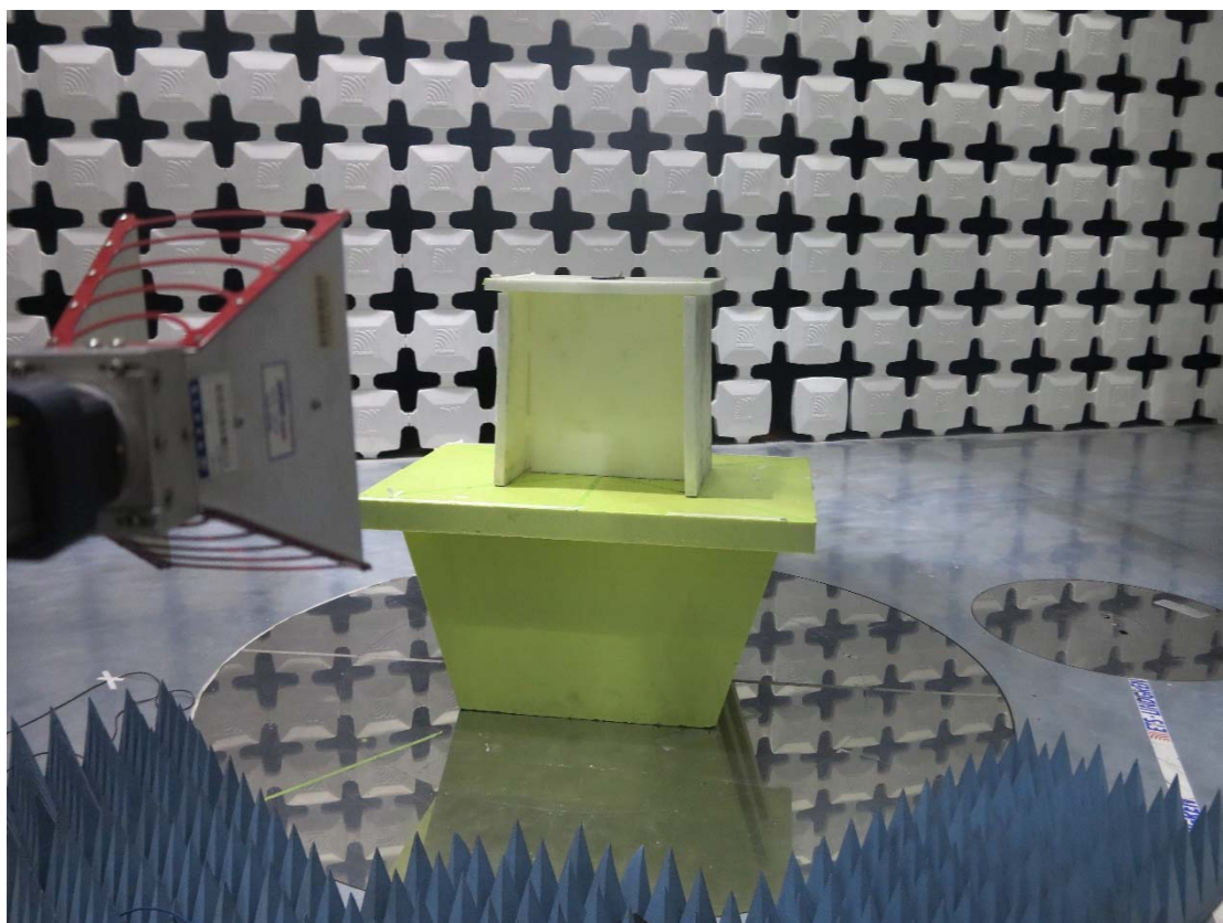
Spurious Emission
