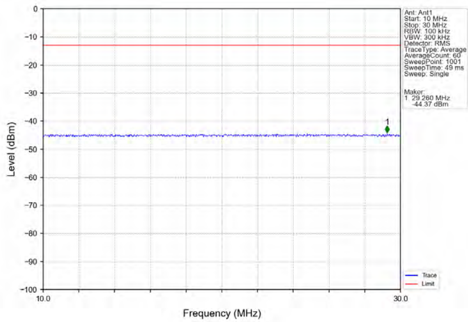
41_Single_NTNV_CC1:20MHz_16QAM_CC1:2680MHz_Ant1
