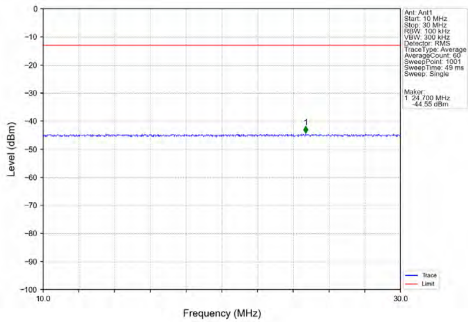
41_Single_NTNV_CC1:20MHz_64QAM_CC1:2680MHz_Ant1
