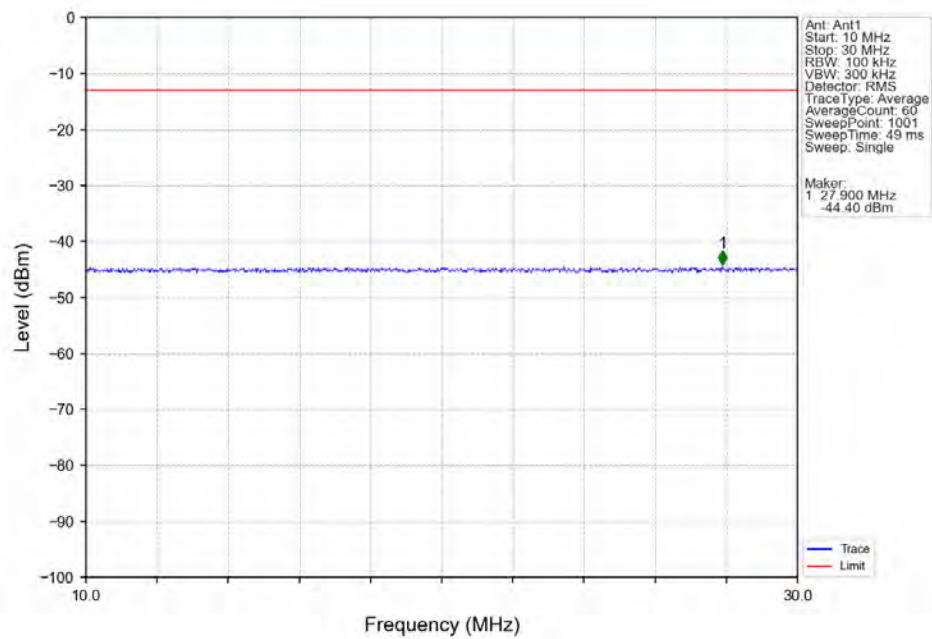
41_Single_NTNV_CC1:20MHz_16QAM_CC1:2593MHz_Ant1
