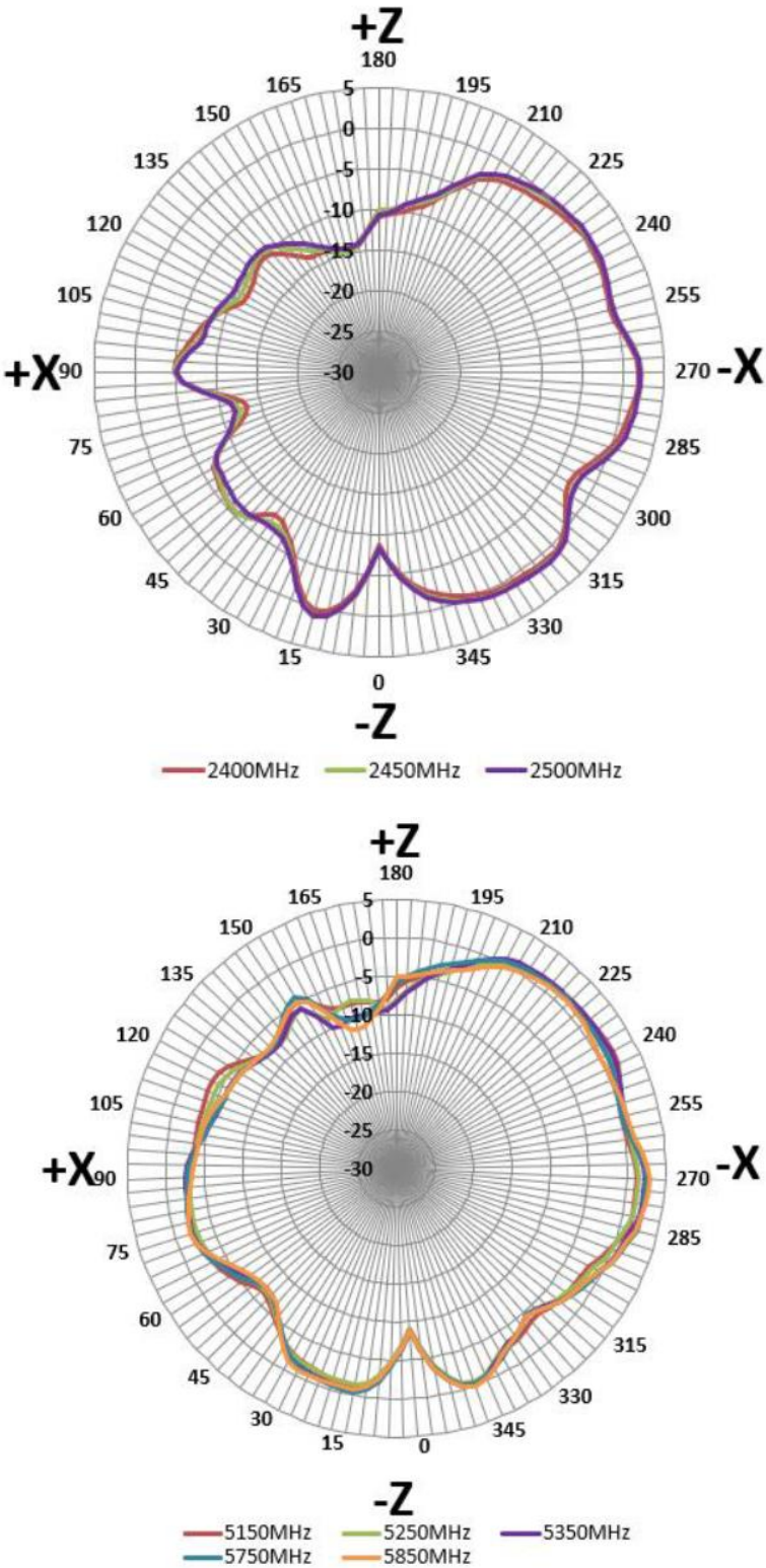
(B). Elevation 1 plane (XZ plane) radiation pattern
