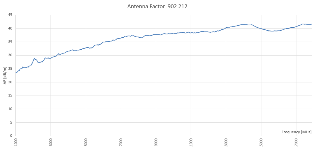
Figure 2: Antenna Factor.
