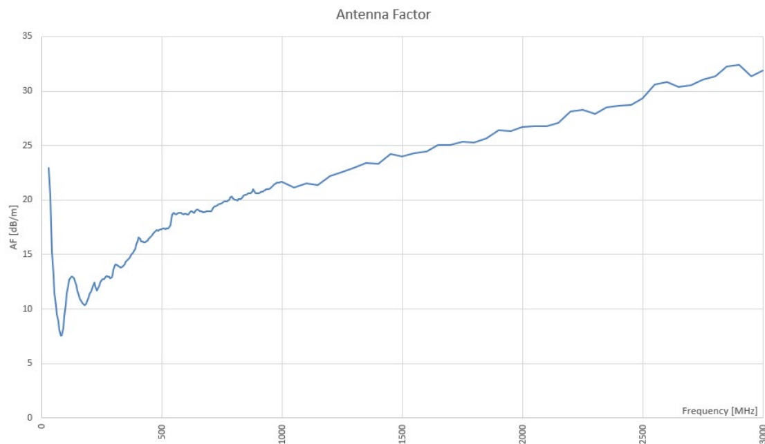
Figure 1: Antenna Factor
