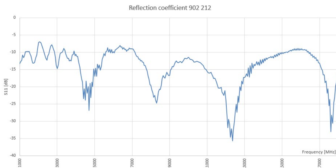
Figure 4: Reflection coefficient
