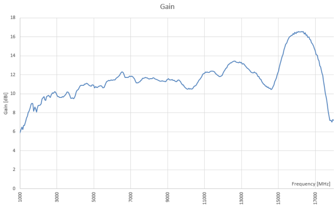
Figure 1: Antenna Gain.
