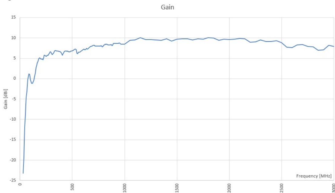
Figure 2: Antenna Gain
