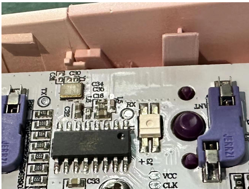
Internal photos M/N: 701
