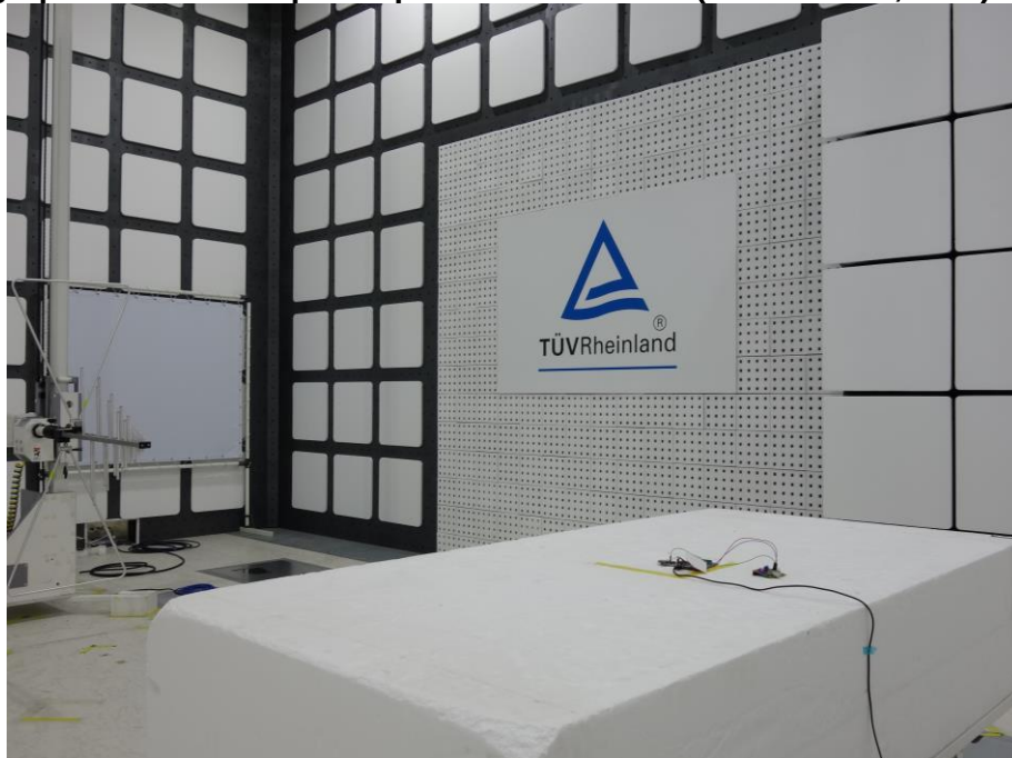
Photograph 12: Test Setup for Spurious Emissions (Back View 2, WiFi)
