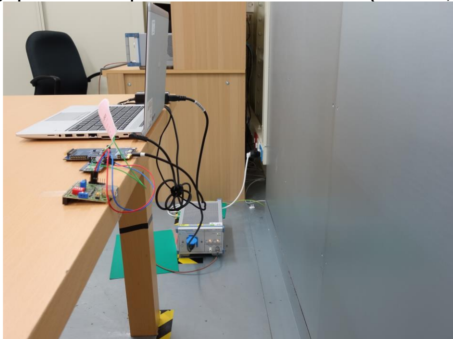
Photograph 16: Test Setup for Mains Conducted Emissions (Back View, WiFi)
