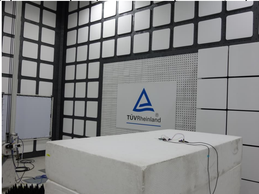
Photograph 6: Test Setup for Spurious Emissions (Back View 4, BLE)
