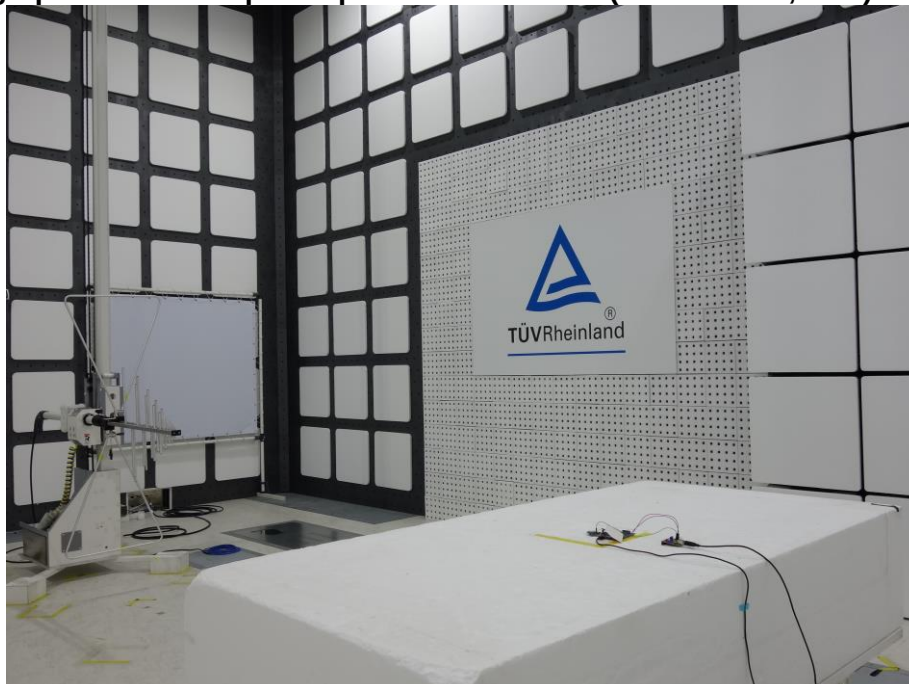
Photograph 4: Test Setup for Spurious Emissions (Back View 2, BLE)
