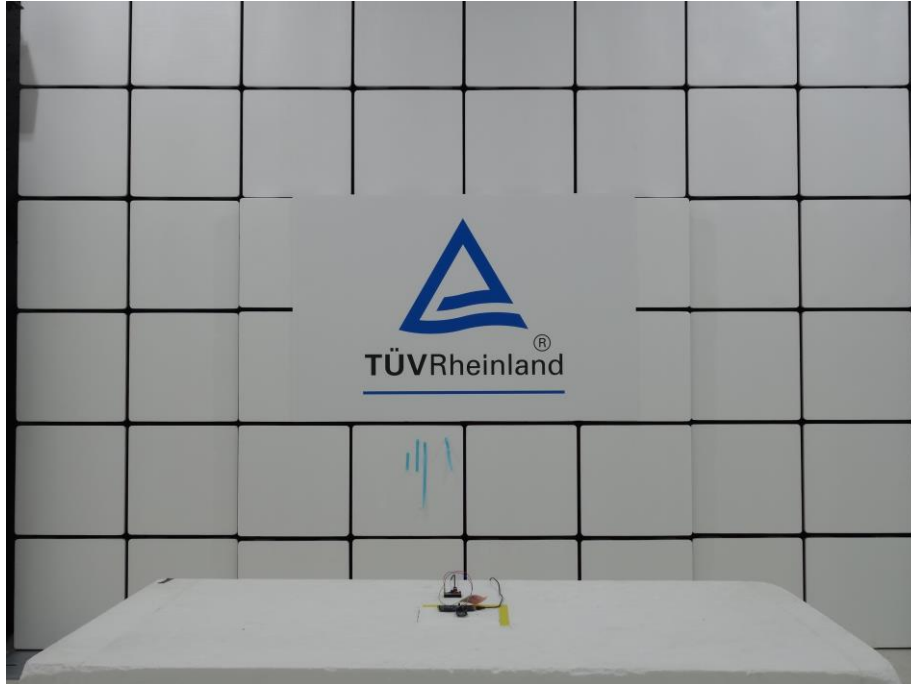
Photograph 1: Test Setup for Spurious Emissions (Front View 1, BLE)
