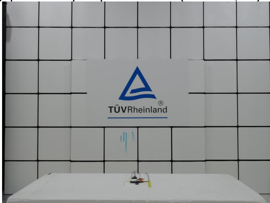
Photograph 2: Test Setup for Spurious Emissions (Front View 2, BLE)
