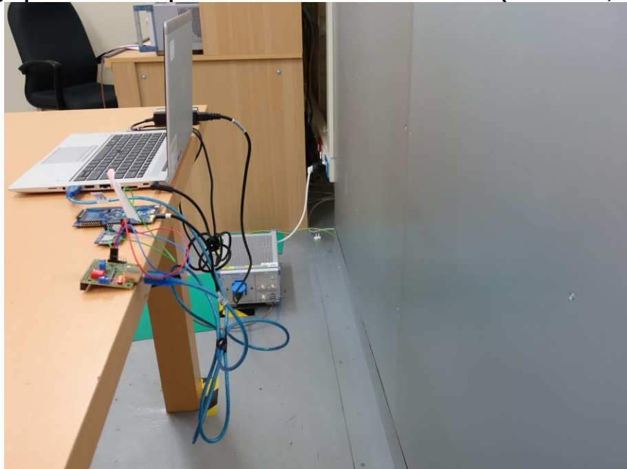
Photograph 8: Test Setup for Mains Conducted Emissions (Back View, BLE)
