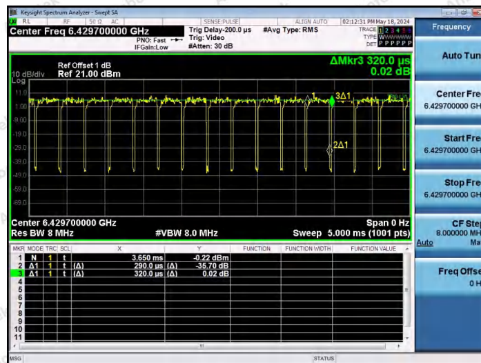
NTNV-11AX40SISO-Ant1-6445-106Tone-RU53
