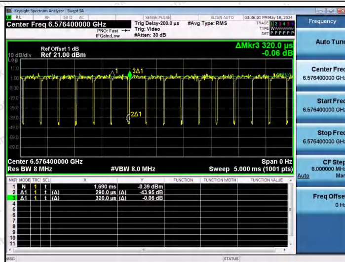
NTNV-11AX40SISO-Ant1-6565-106Tone-RU56
