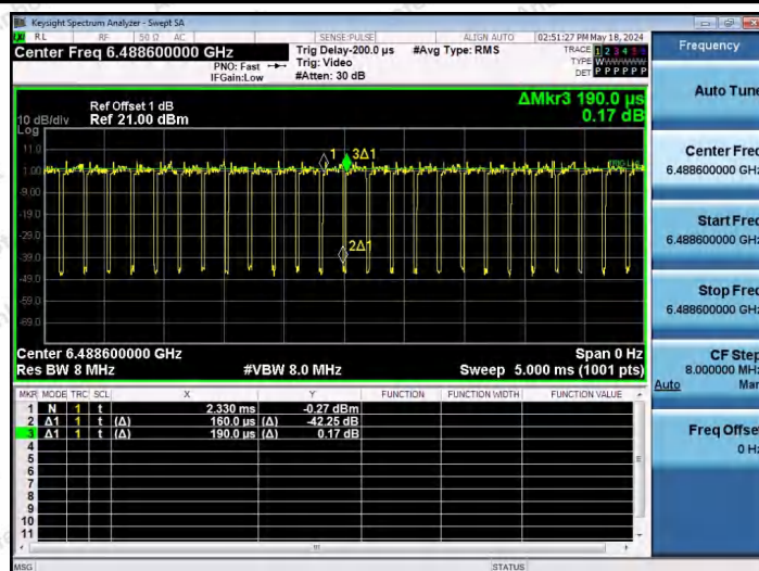
NTNV-11AX40SISO-Ant1-6485-242Tone-RU62
