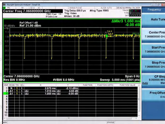
NTNV-11AX40SISO-Ant1-7085-26Tone-RU0
