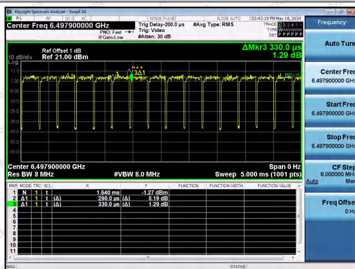
NTNV-11AX40SISO-Ant1-6485-106Tone-RU56
