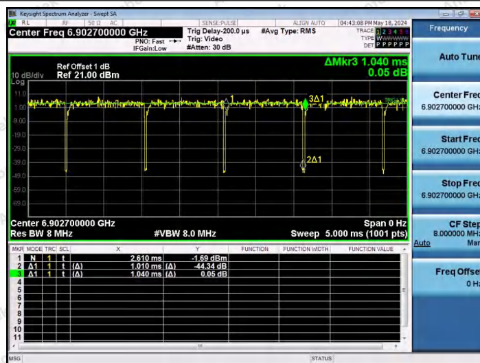
NTNV-11AX40SISO-Ant1-6885-26Tone-RU17
