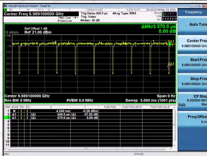
NTNV-11AX40SISO-Ant1-7005-52Tone-RU37
