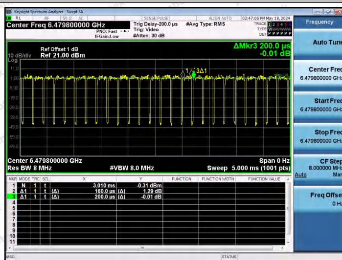
NTNV-11AX40SISO-Ant1-6485-242Tone-RU61
