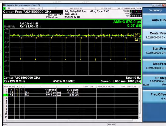
NTNV-11AX40SISO-Ant1-7005-52Tone-RU44
