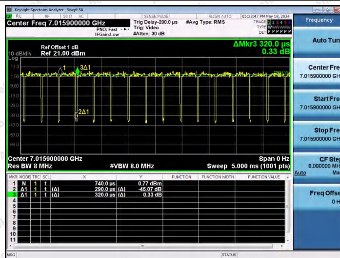
NTNV-11AX40SISO-Ant1-7005-106Tone-RU56
