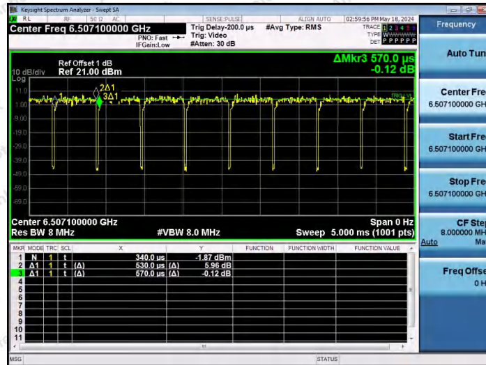
NTNV-11AX40SISO-Ant1-6525-52Tone-RU37
