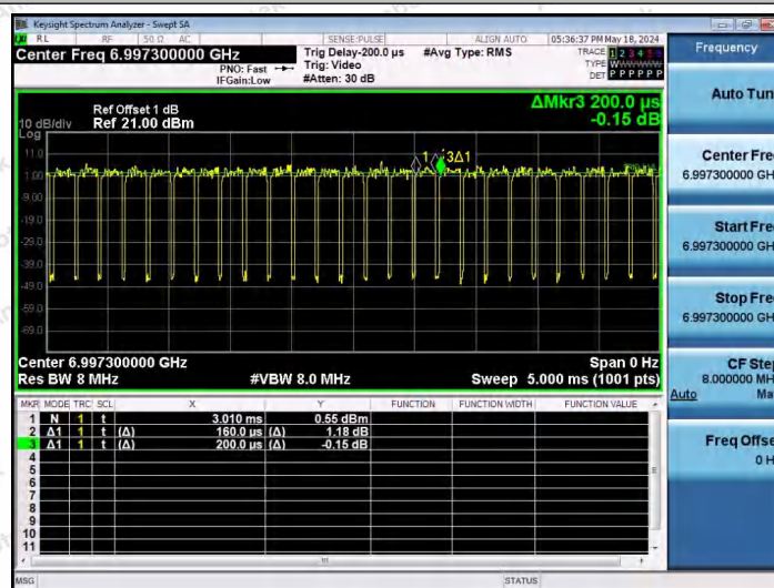
NTNV-11AX40SISO-Ant1-7005-242Tone-RU61
