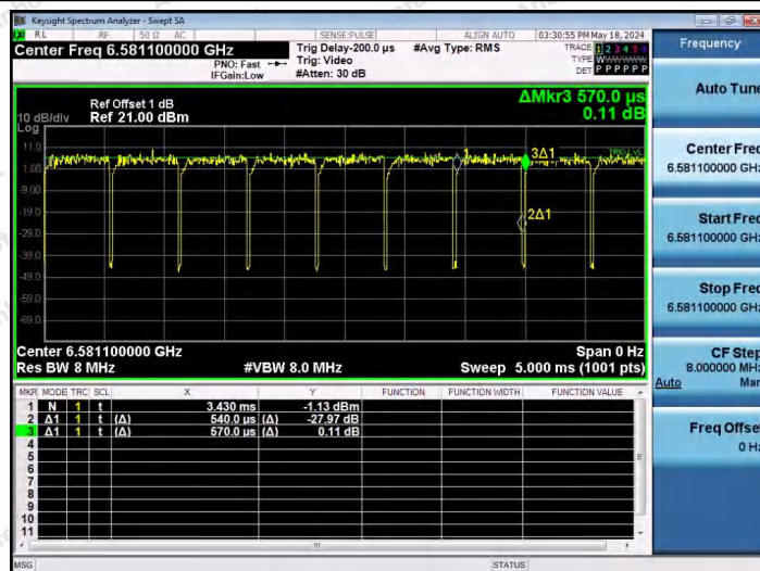
NTNV-11AX40SISO-Ant1-6565-52Tone-RU44
