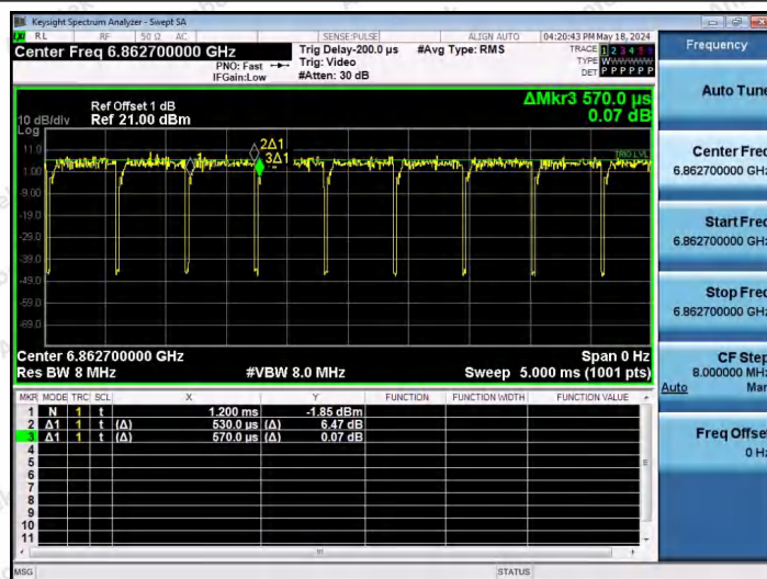
NTNV-11AX40SISO-Ant1-6845-52Tone-RU44
