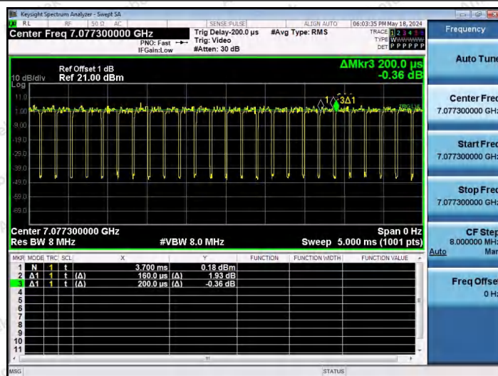
NTNV-11AX40SISO-Ant1-7085-242Tone-RU61
