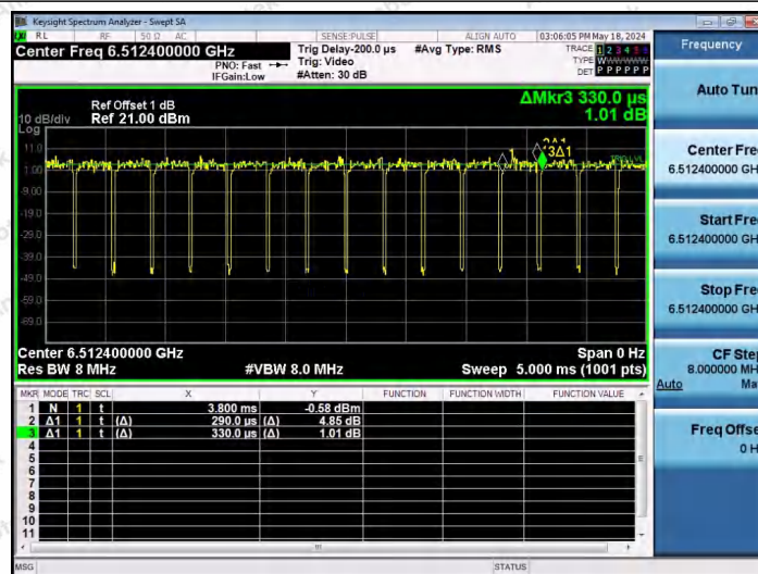
NTNV-11AX40SISO-Ant1-6525-106Tone-RU53
