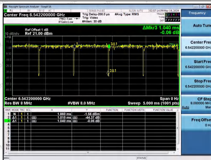
NTNV-11AX40SISO-Ant1-6525-26Tone-RU17
