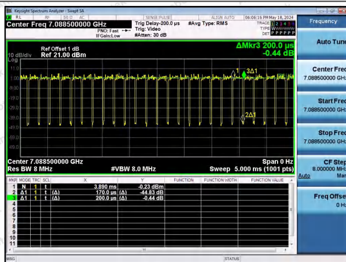
NTNV-11AX40SISO-Ant1-7085-242Tone-RU62
