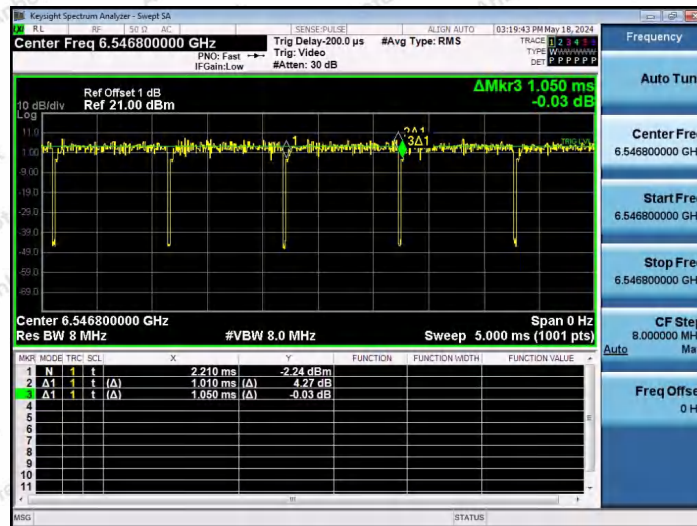
NTNV-11AX40SISO-Ant1-6565-26Tone-RU0
