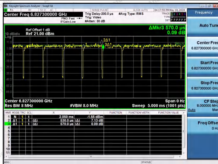
NTNV-11AX40SISO-Ant1-6845-52Tone-RU37
