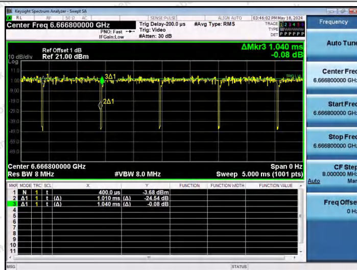
NTNV-11AX40SISO-Ant1-6685-26Tone-RU0
