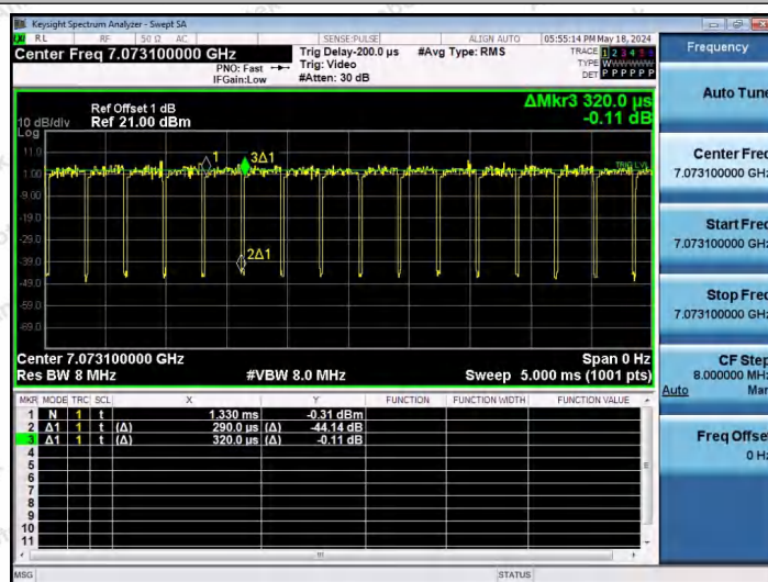
NTNV-11AX40SISO-Ant1-7085-106Tone-RU53
