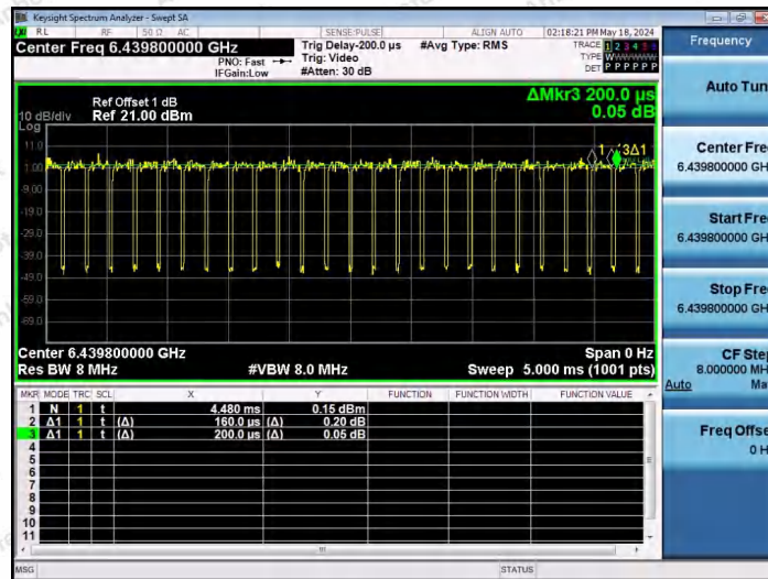
NTNV-11AX40SISO-Ant1-6445-242Tone-RU61
