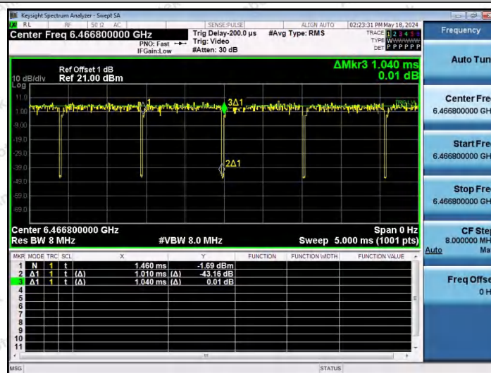
NTNV-11AX40SISO-Ant1-6485-26Tone-RU0
