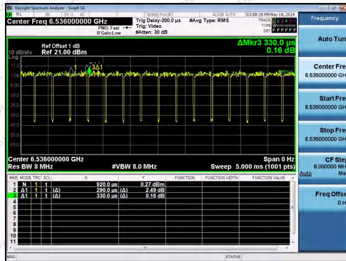
NTNV-11AX40SISO-Ant1-6525-106Tone-RU56
