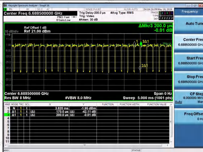
NTNV-11AX40SISO-Ant1-6685-242Tone-RU62
