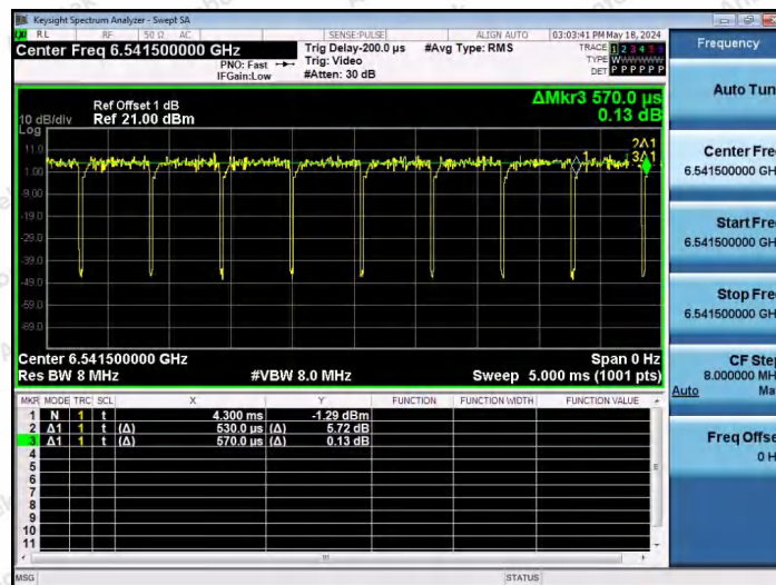
NTNV-11AX40SISO-Ant1-6525-52Tone-RU44
