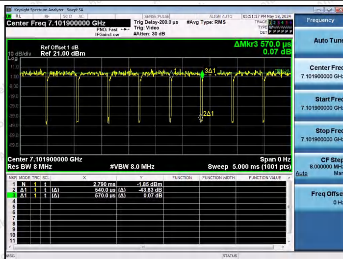
NTNV-11AX40SISO-Ant1-7085-52Tone-RU44
