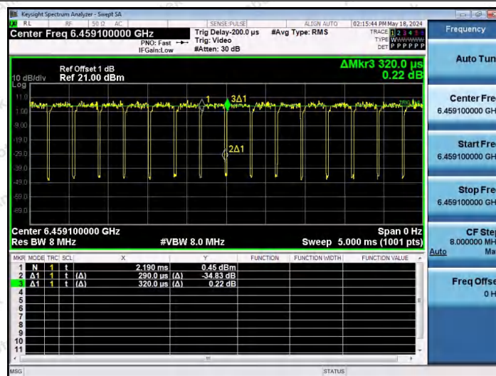
NTNV-11AX40SISO-Ant1-6445-106Tone-RU56
