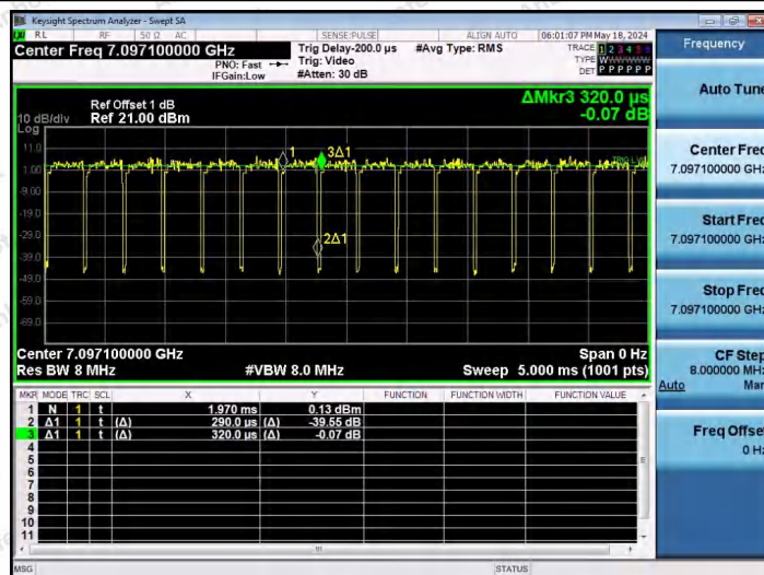
NTNV-11AX40SISO-Ant1-7085-106Tone-RU56
