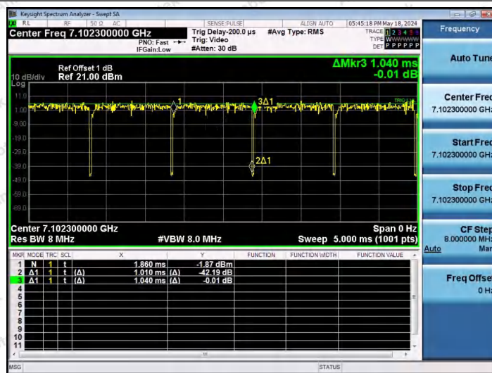
NTNV-11AX40SISO-Ant1-7085-26Tone-RU17
