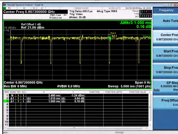
NTNV-11AX40SISO-Ant1-6885-26Tone-RU0
