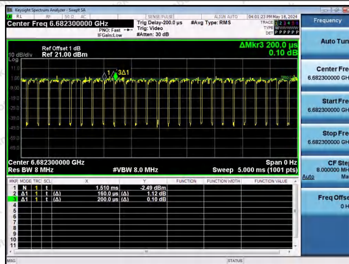
NTNV-11AX40SISO-Ant1-6685-242Tone-RU61
