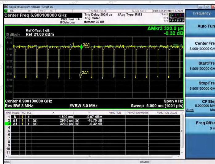
NTNV-11AX40SISO-Ant1-6885-106Tone-RU56
