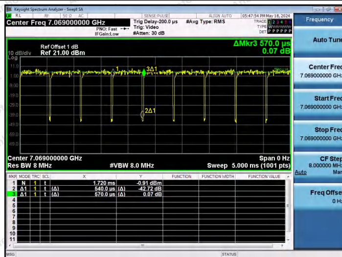
NTNV-11AX40SISO-Ant1-7085-52Tone-RU37
