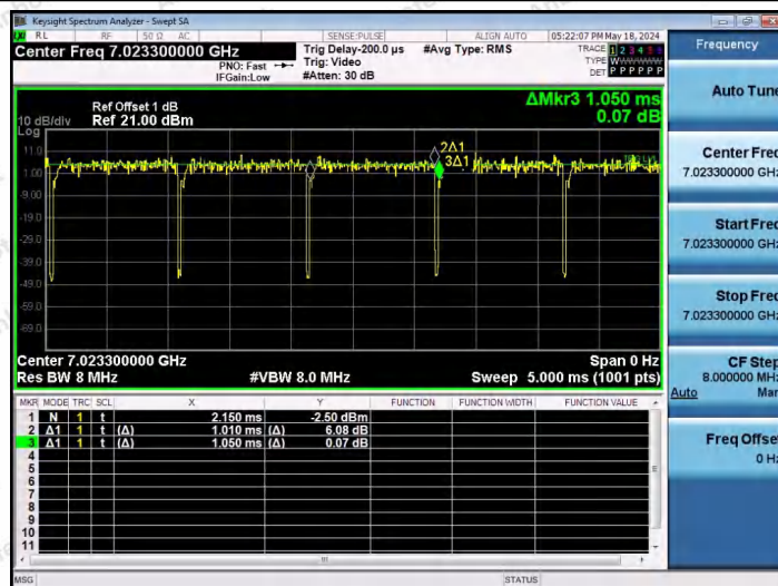
NTNV-11AX40SISO-Ant1-7005-26Tone-RU17
