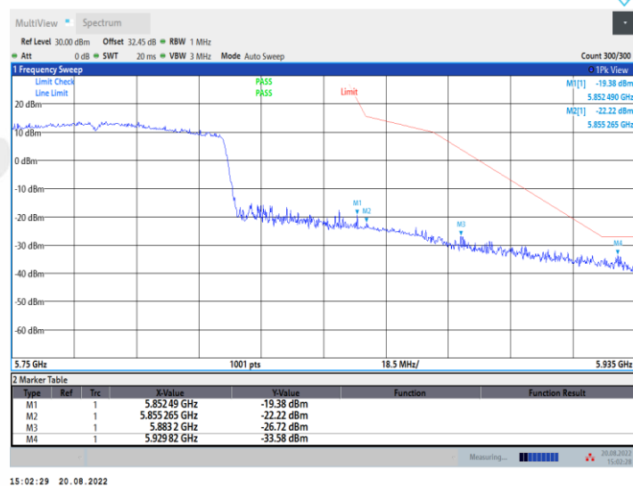
11AC80SISO_Ant1_High_5775
