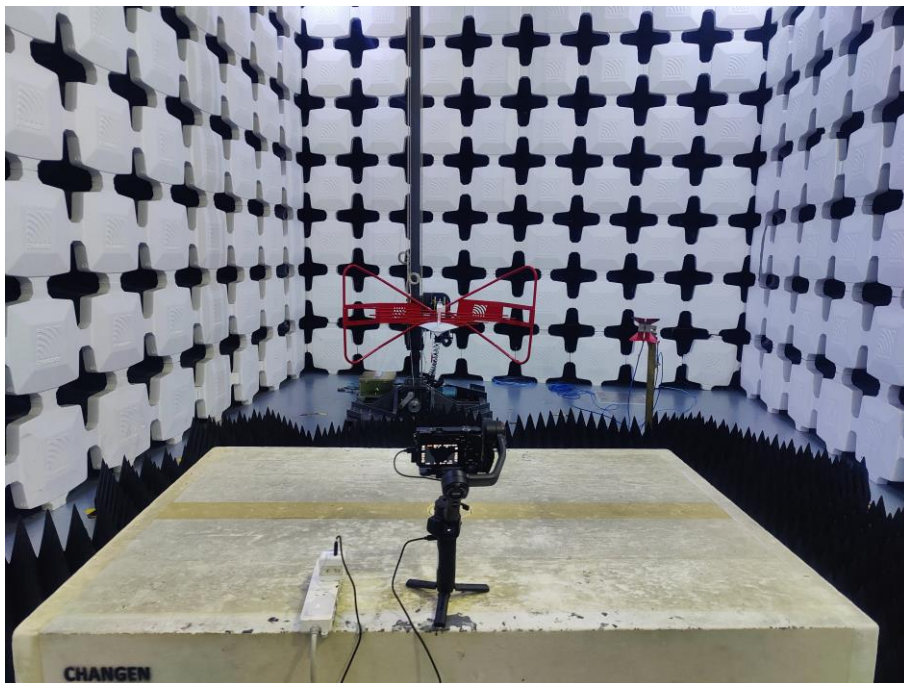
2. Radiated Emissions (Part 15B Normal Working, 1GHz-18GHz)
