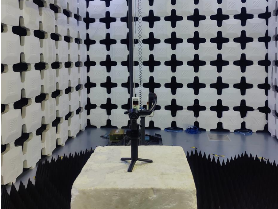
7. Radiated Emissions (Part 15C Bluetooth, 18GHz -26.5GHz)
