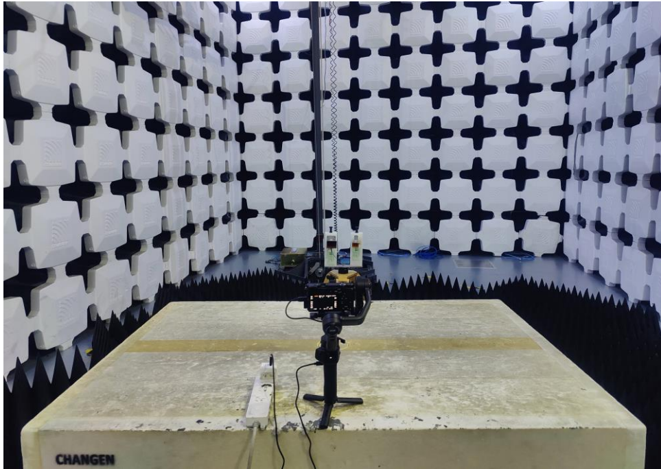
3. Radiated Emissions (Part 15B Normal Working, 18GHz-26.5GHz)
