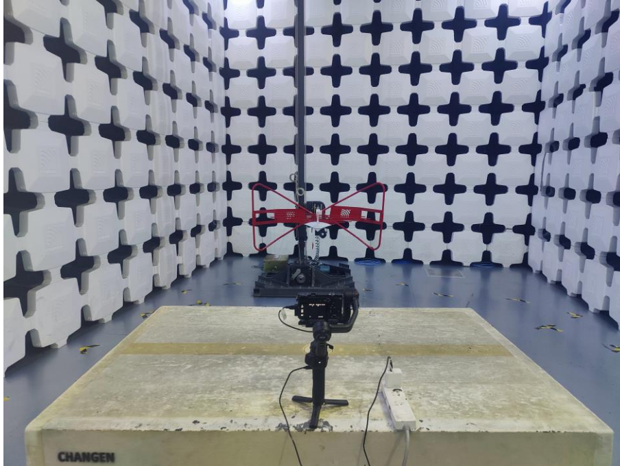
1. Radiated Emissions (Part 15B Normal Working, 30MHz-1GHz)
