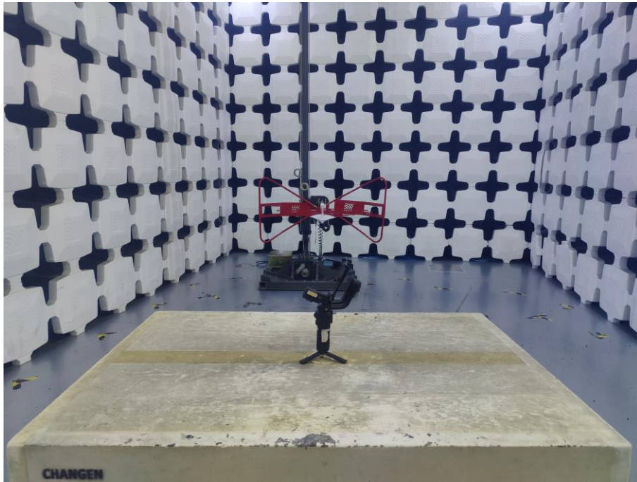
5. Radiated Emissions (Part 15C Bluetooth, 30MHz-1GHz)
