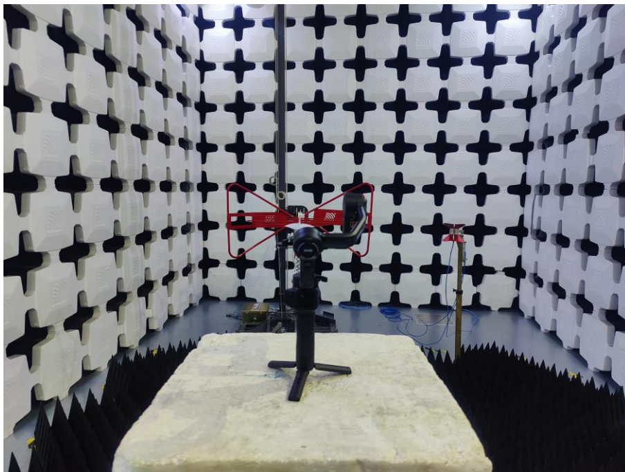
6. Radiated Emissions (Part 15C Bluetooth, 1GHz -18GHz)
