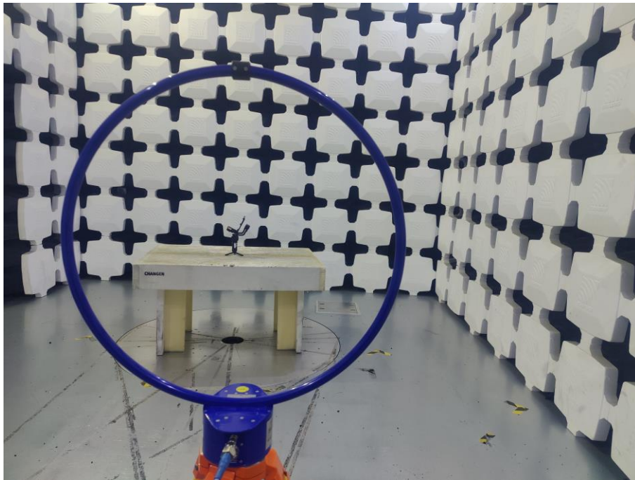
4. Radiated Emissions (Part 15C Bluetooth, 9kHz-30MHz)
