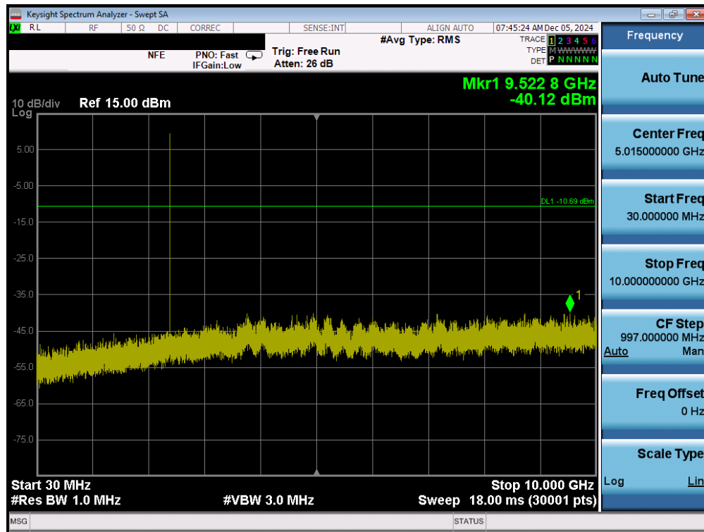
Plot 7-95. Conducted Spurious Plot (Bluetooth (LE), 1Mbps – Ch. 37) – Ant 2
