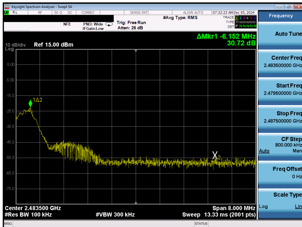
Plot 7-80. Band Edge Plot (Bluetooth (LE), 2Mbps – Ch. 36) – Ant 1
