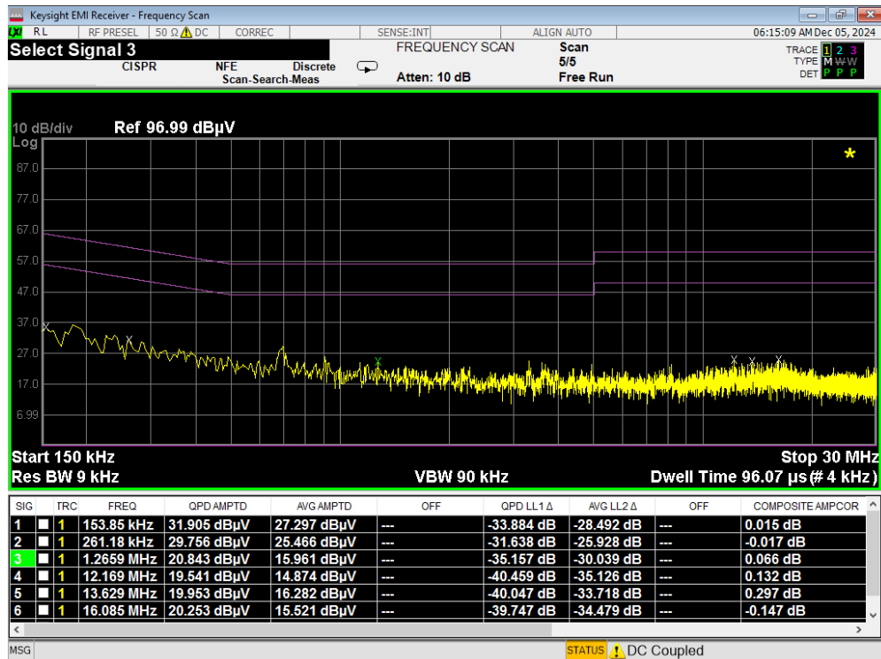
Plot 7-115. Line Conducted Plot with Bluetooth LE (L1) - WCP
