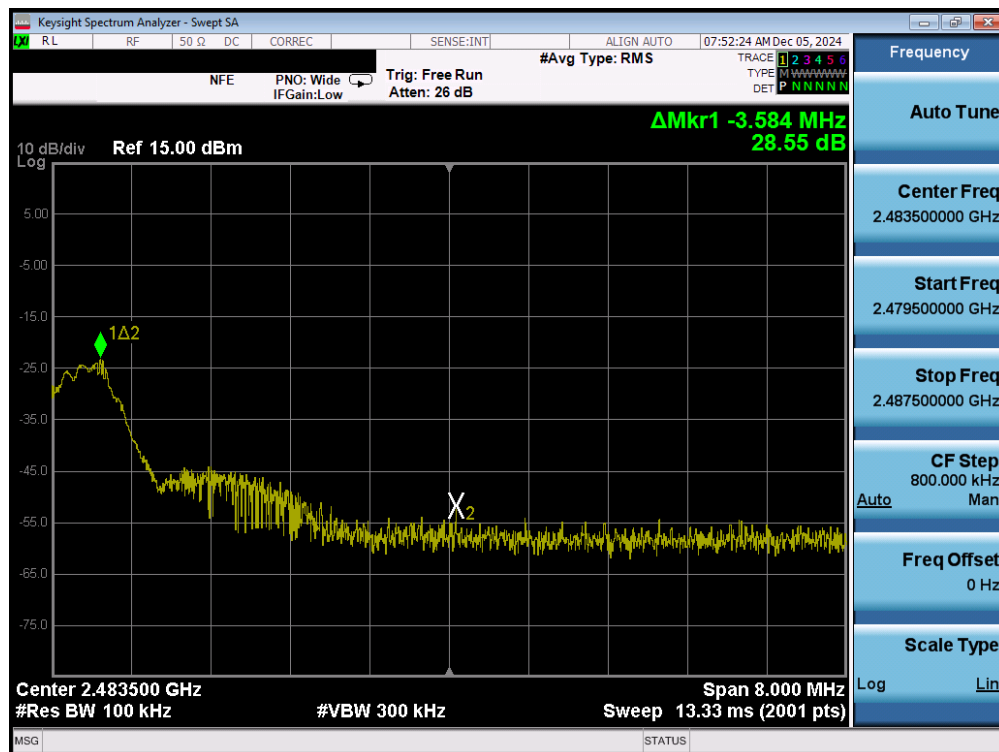
Plot 7-88. Band Edge Plot (Bluetooth (LE), 2Mbps – Ch. 36) – Ant 2
