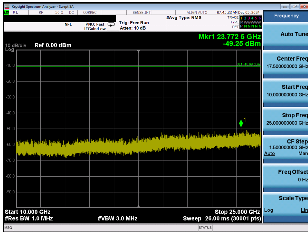
Plot 7-96. Conducted Spurious Plot (Bluetooth (LE), 1Mbps – Ch. 37) – Ant 2
