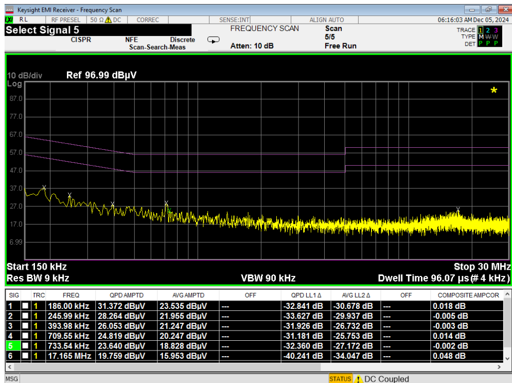
Plot 7-116. Line Conducted Plot with Bluetooth LE (N) - WCP
