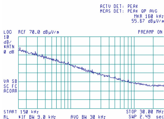
Plot 8.4.6 Radiated emission measurements from 0.15 to 30 MHz at the high carrier frequency
