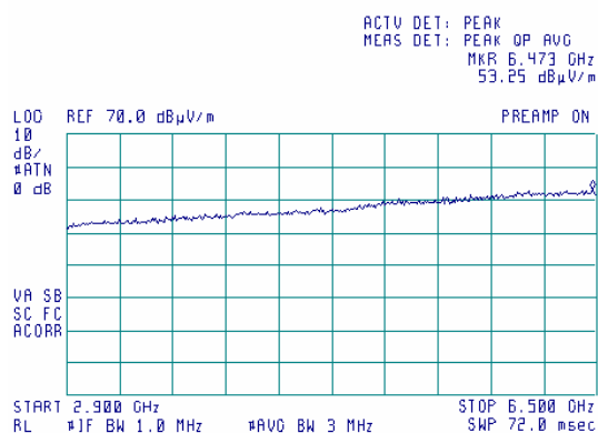
Plot 8.4.14 Radiated emission measurements from 2900 to 6500 MHz at the mid carrier frequency
