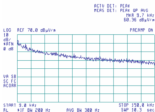
Plot 8.4.2 Radiated emission measurements from 9 to 150 kHz at the mid carrier frequency
