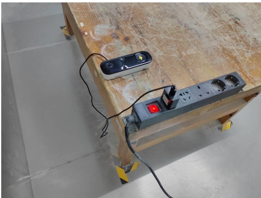
Conducted Emissions Side View- AC/DC Adapter power
