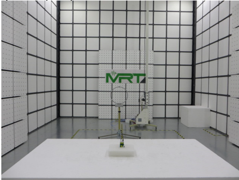
Photograph 2: Set-up for Spurious Emissions below 1GHz
